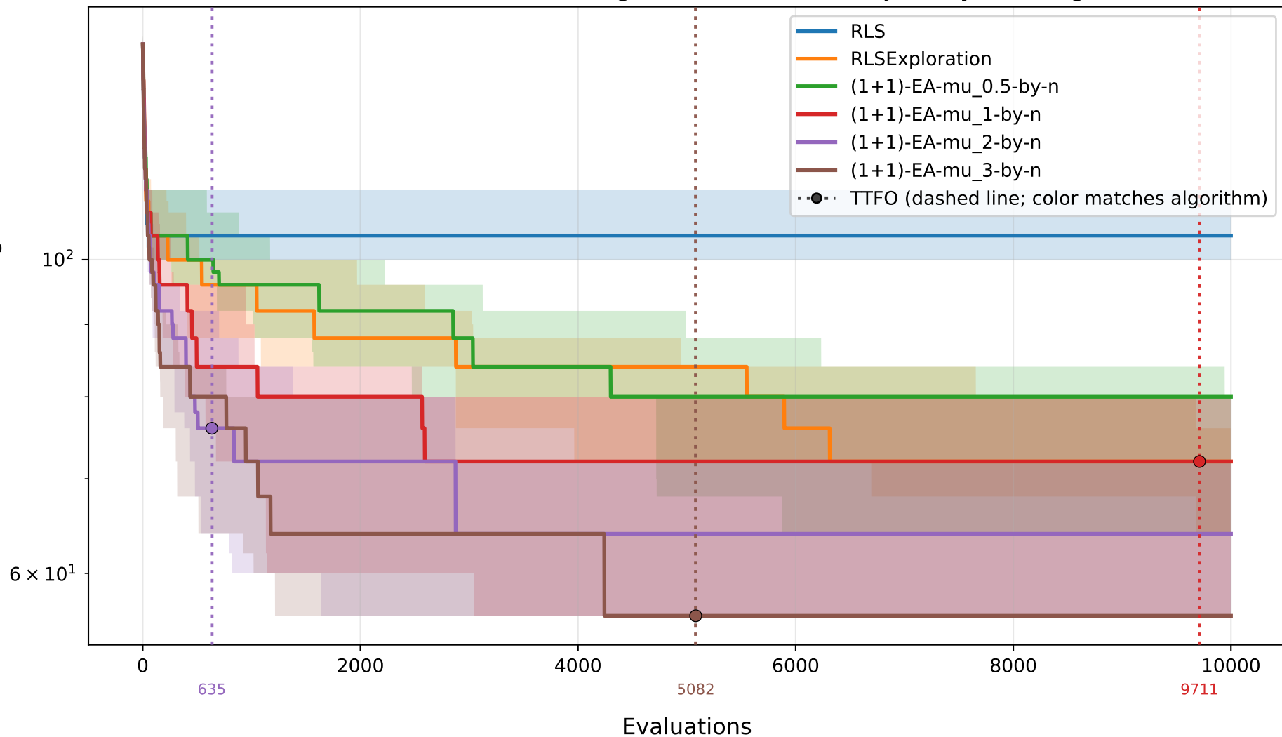
HIFF-n32 - n=32: Instantaneous Regret (incumbent) Trajectory at Budget=10000
