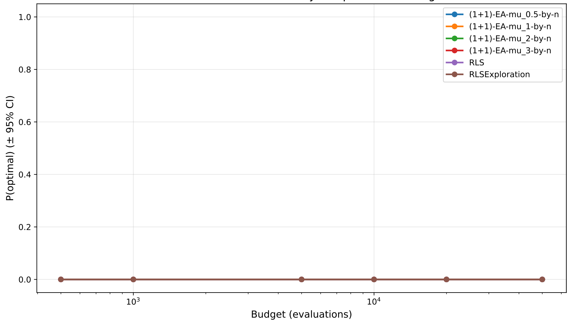
HIFF-n64 - n=64: Probability of Optimum vs Budget
