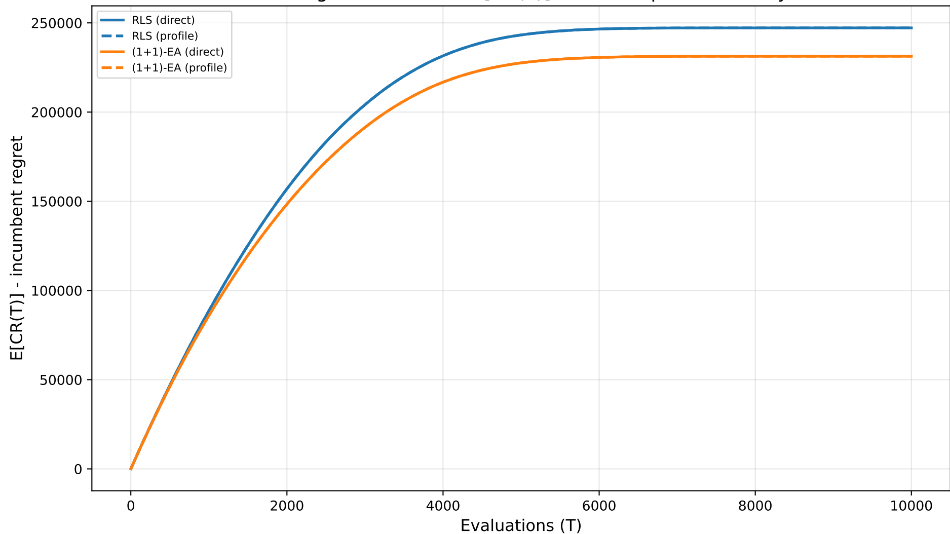
LeadingOnes - n=100 : E[CR(T)] : direct vs profile identity
