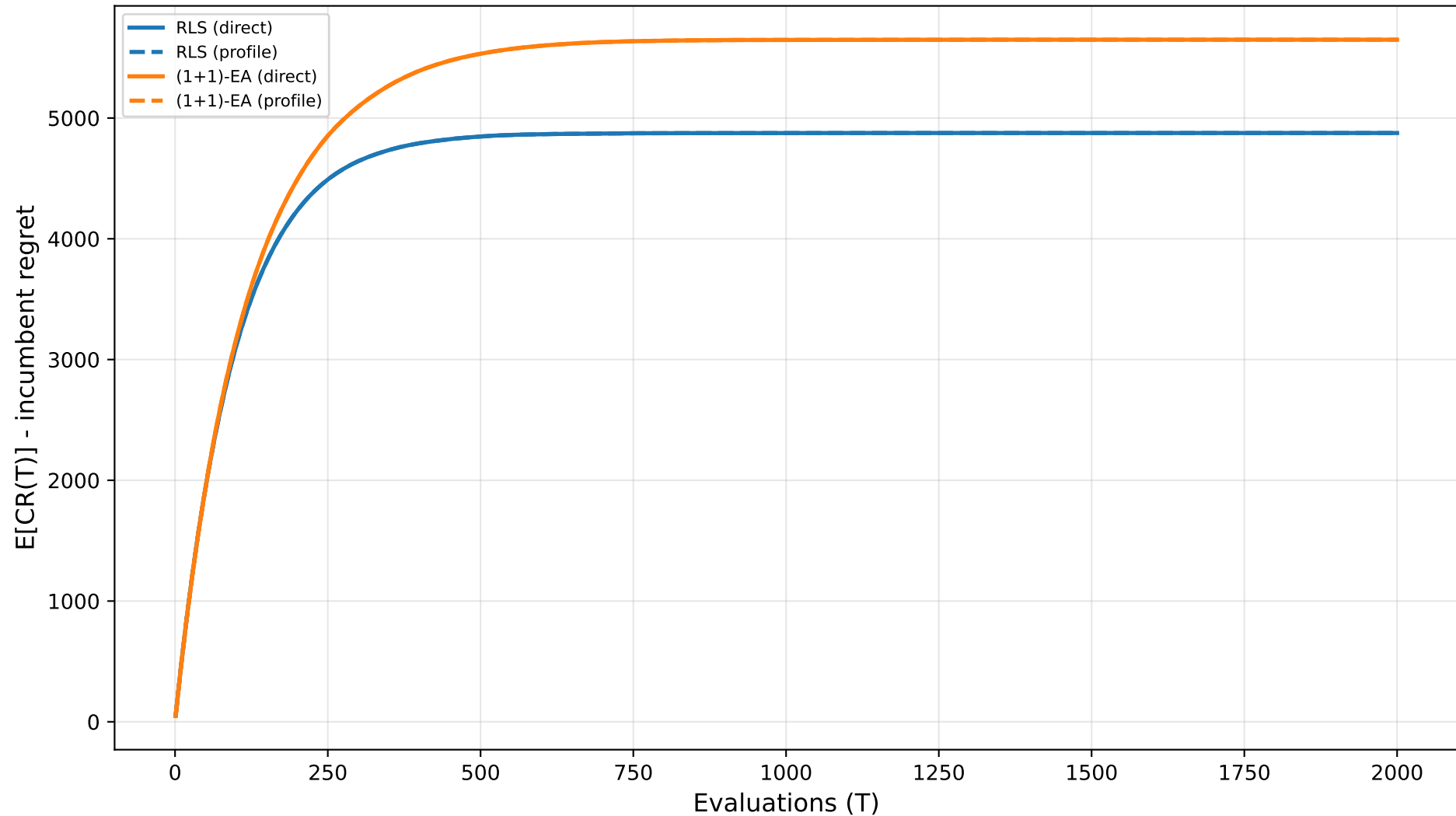
OneMax - n=100 : E[CR(T)] : direct vs profile identity
