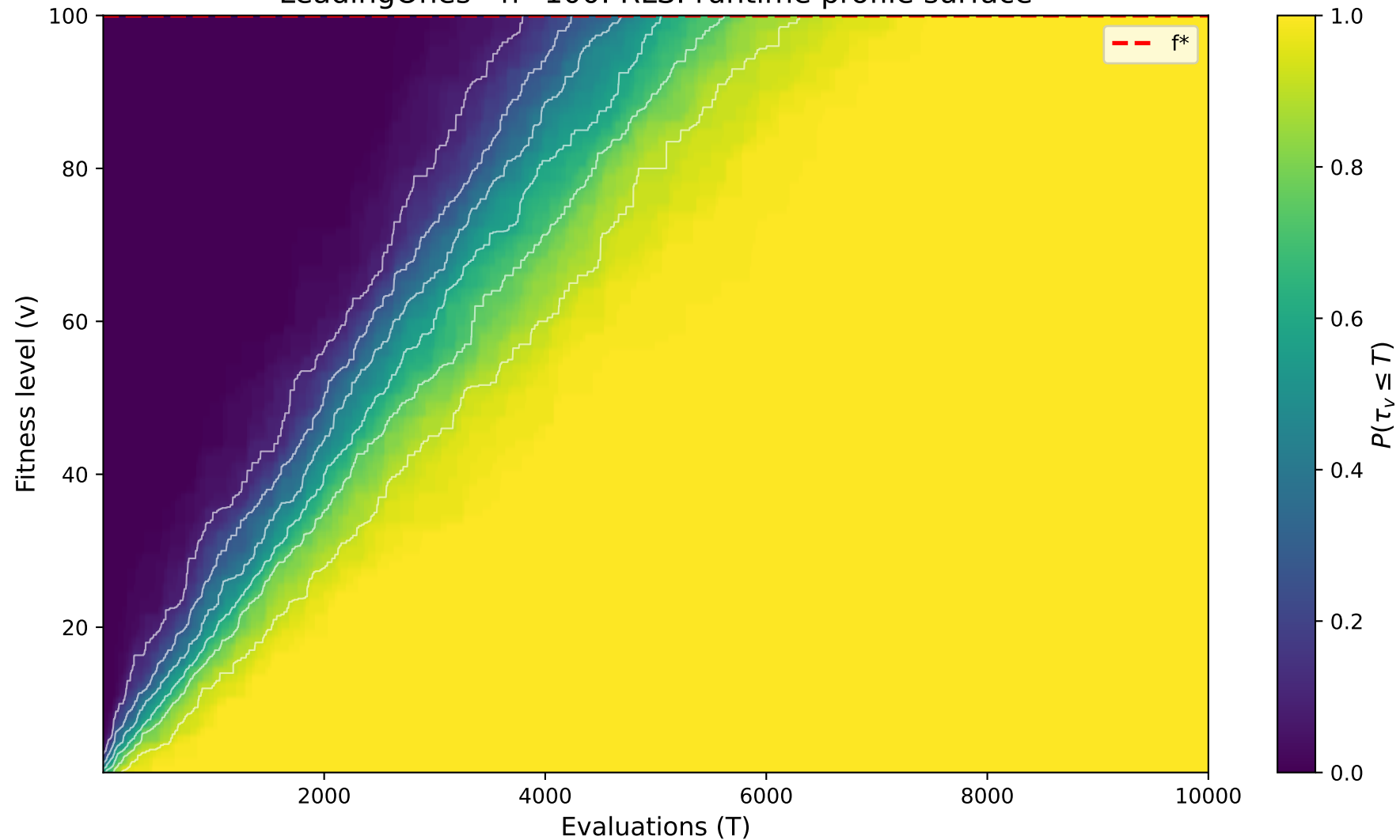
LeadingOnes - n=100: RLS: runtime profile surface
