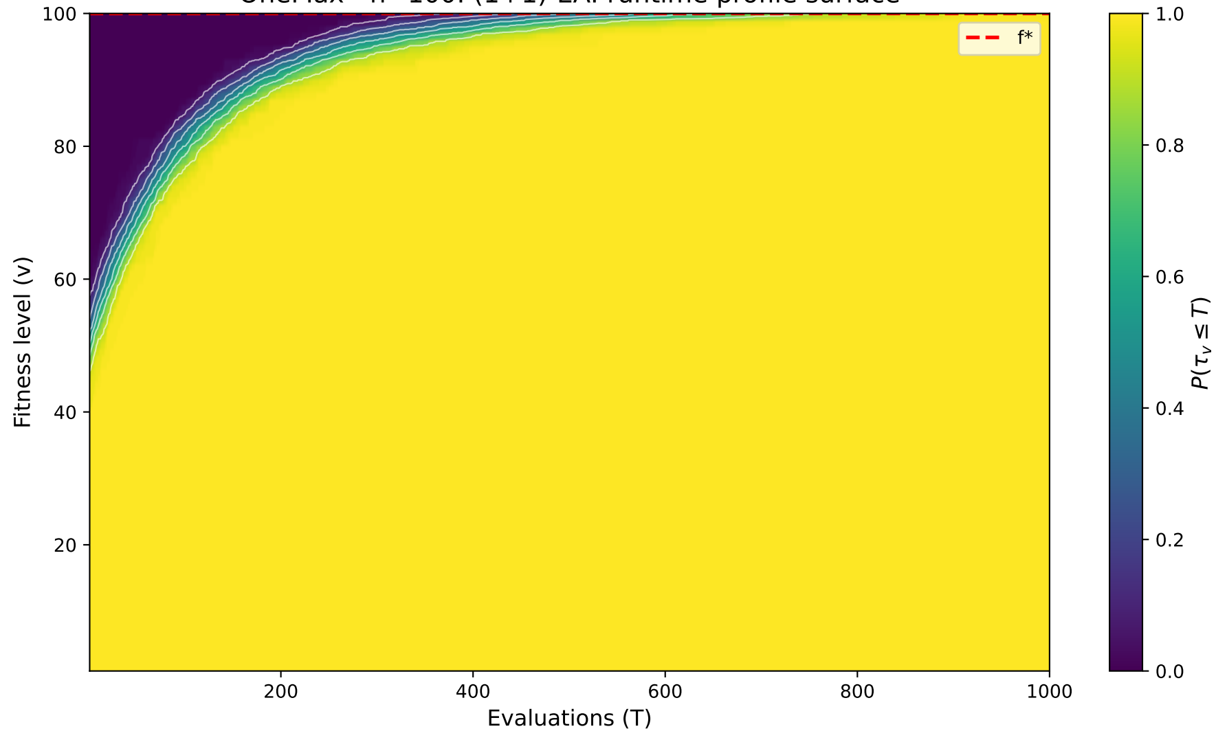
OneMax - n=100: (1+1)-EA: runtime profile surface
