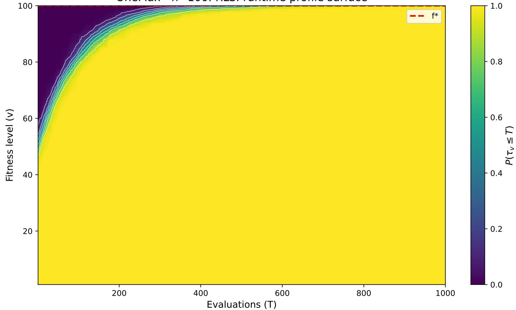
OneMax - n=100: RLS: runtime profile surface
