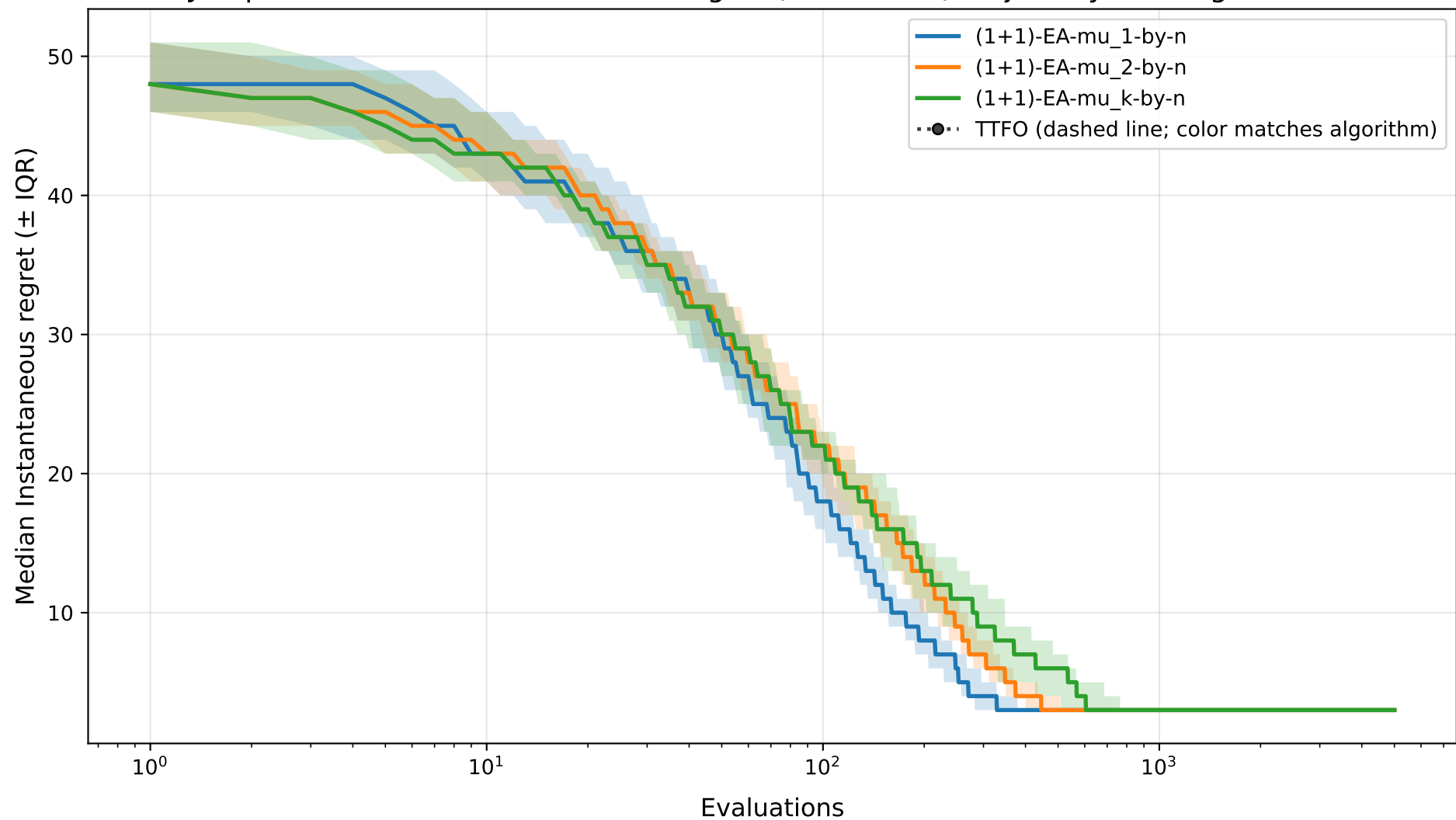
Jump-k3 - n=100: Instantaneous Regret (incumbent) Trajectory at Budget=5000
