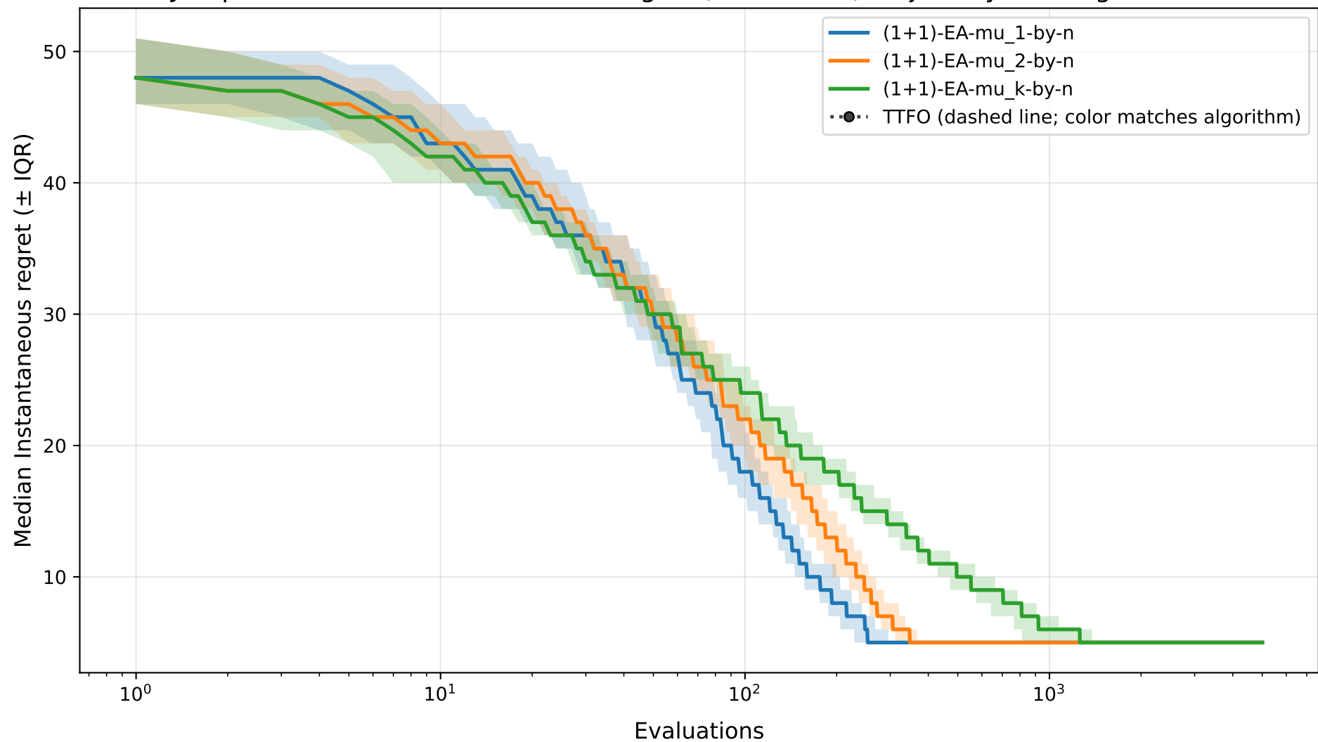
Jump-k5 - n=100: Instantaneous Regret (incumbent) Trajectory at Budget=5000
