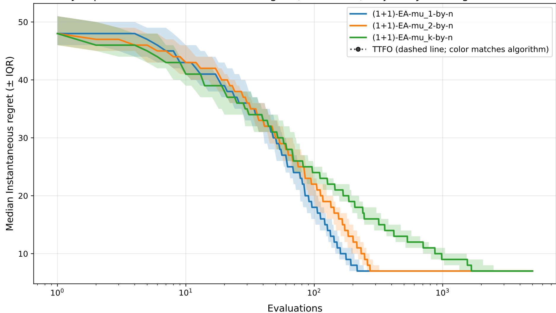
Jump-k7 - n=100: Instantaneous Regret (incumbent) Trajectory at Budget=5000
