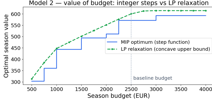
Figure 7: Season value vs. budget: the MIP optimum is a step function; the LP relaxation is a concave upper bound. Beyond 3000 EUR the vacation-days budget becomes binding and money stops mattering.
