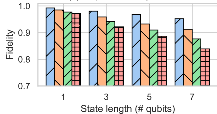
(a) Repeated teleportation
