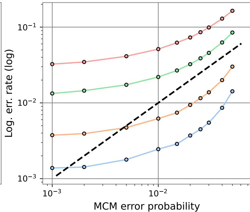
(b) QEC threshold
