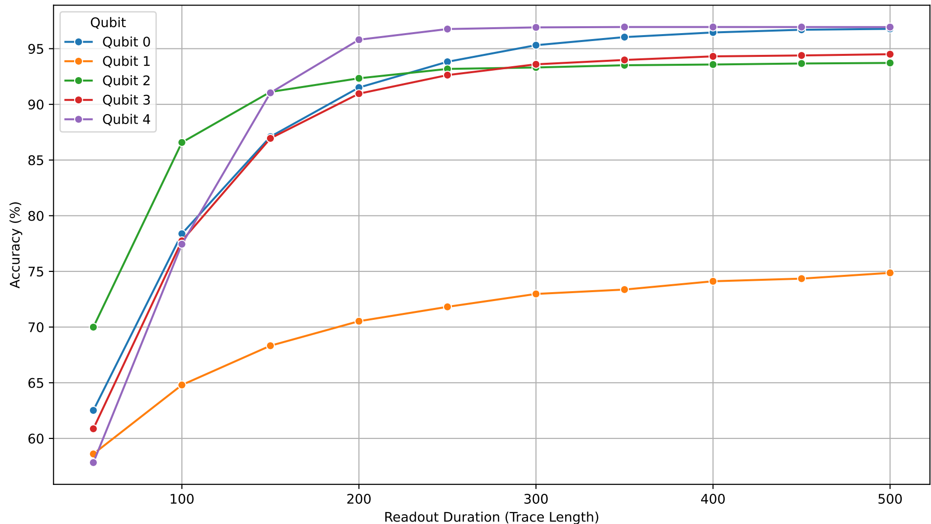
Individual Qubit Accuracies vs Readout Duration (FNN)
