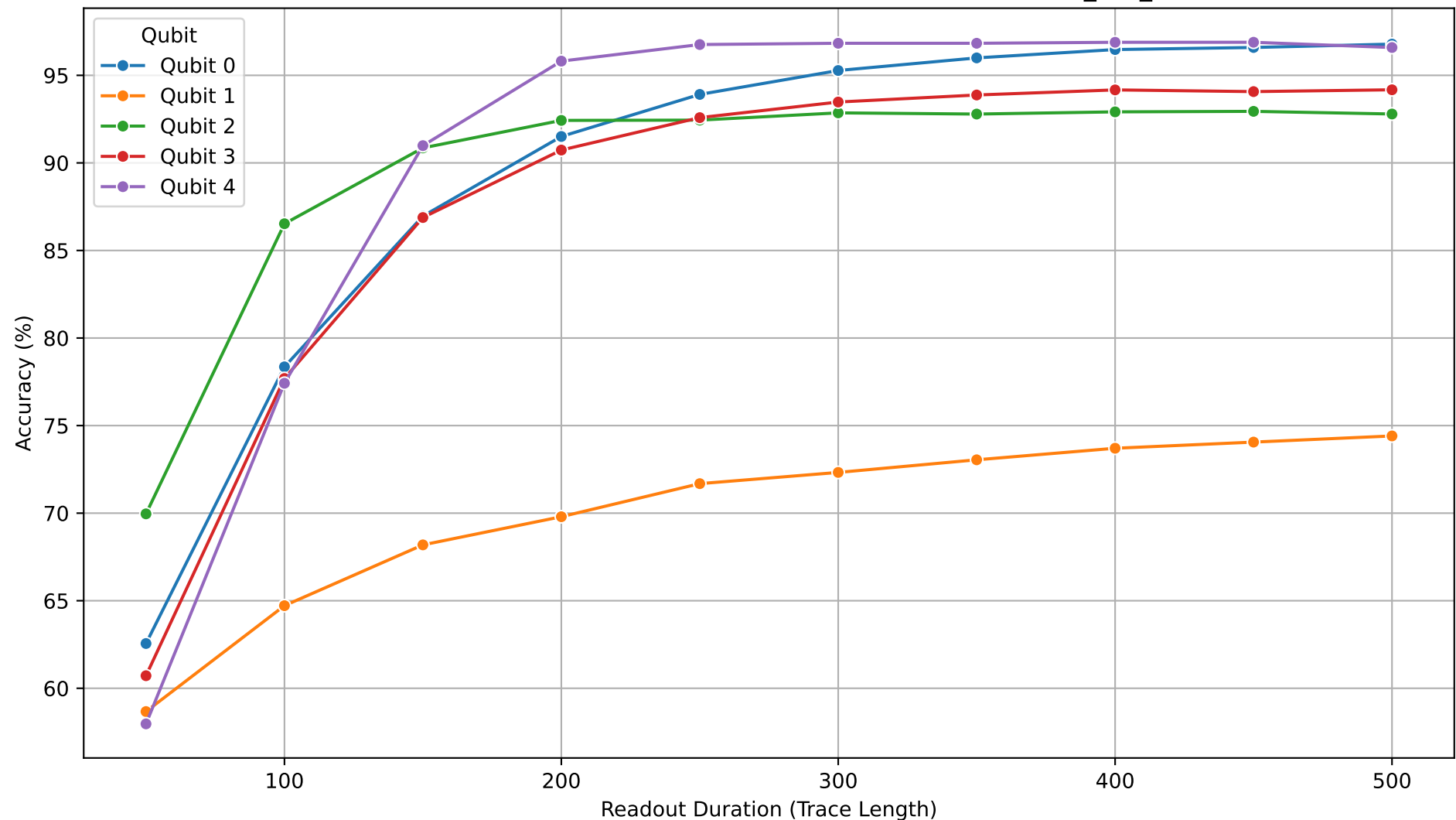
Individual Qubit Accuracies vs Readout Duration (HERQULES_Net_rmf)
