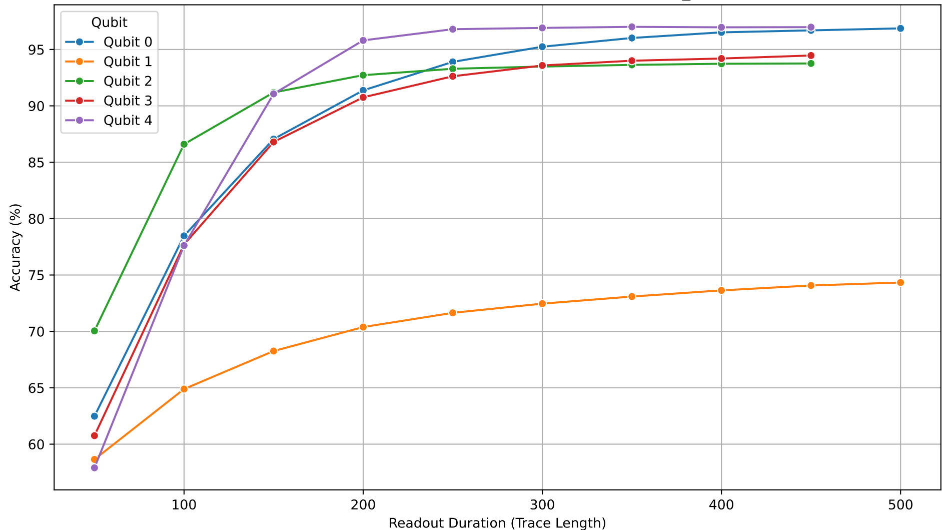
Individual Qubit Accuracies vs Readout Duration (KLiNQ_Student)
