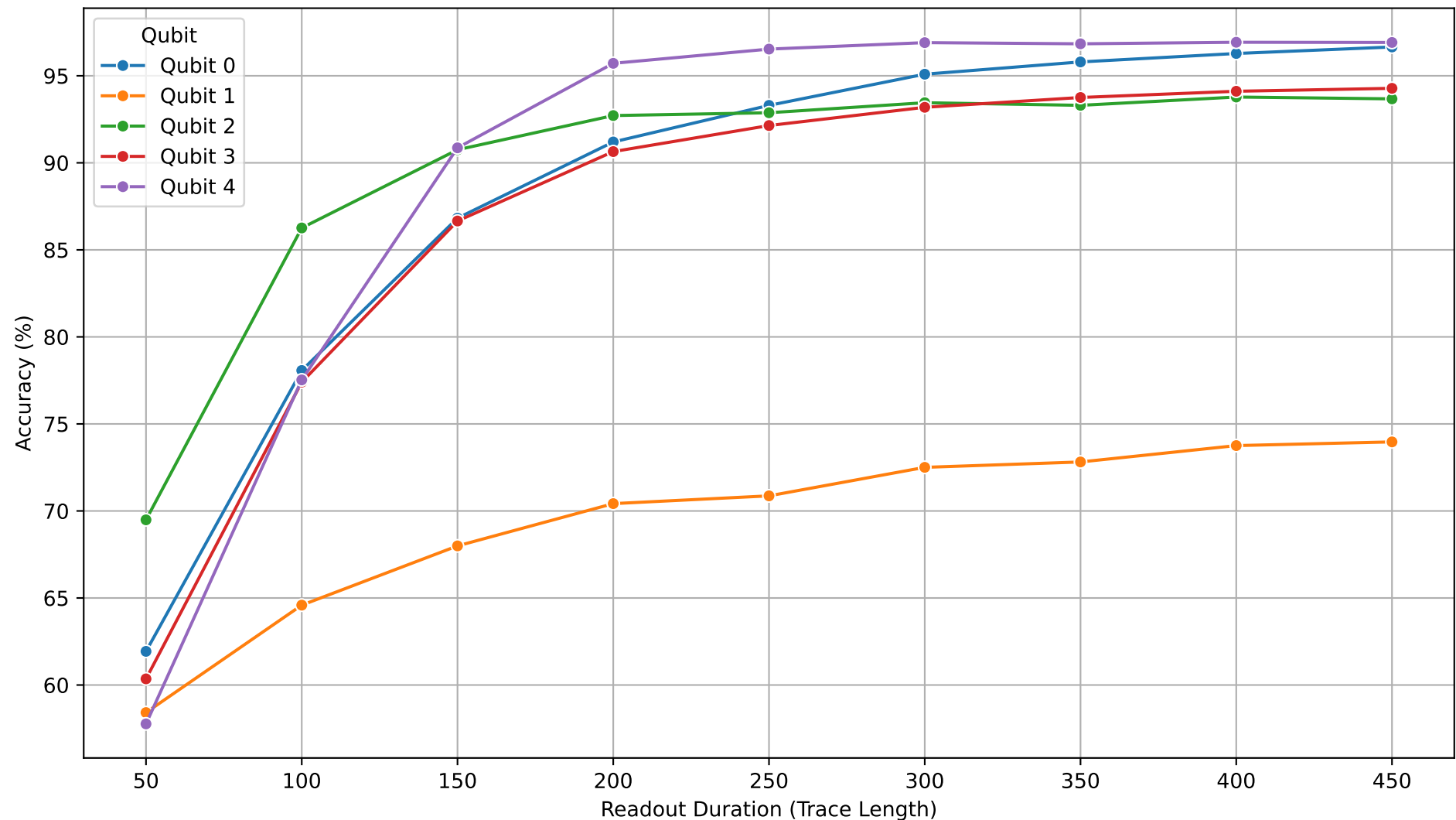
Individual Qubit Accuracies vs Readout Duration (Transformer)
