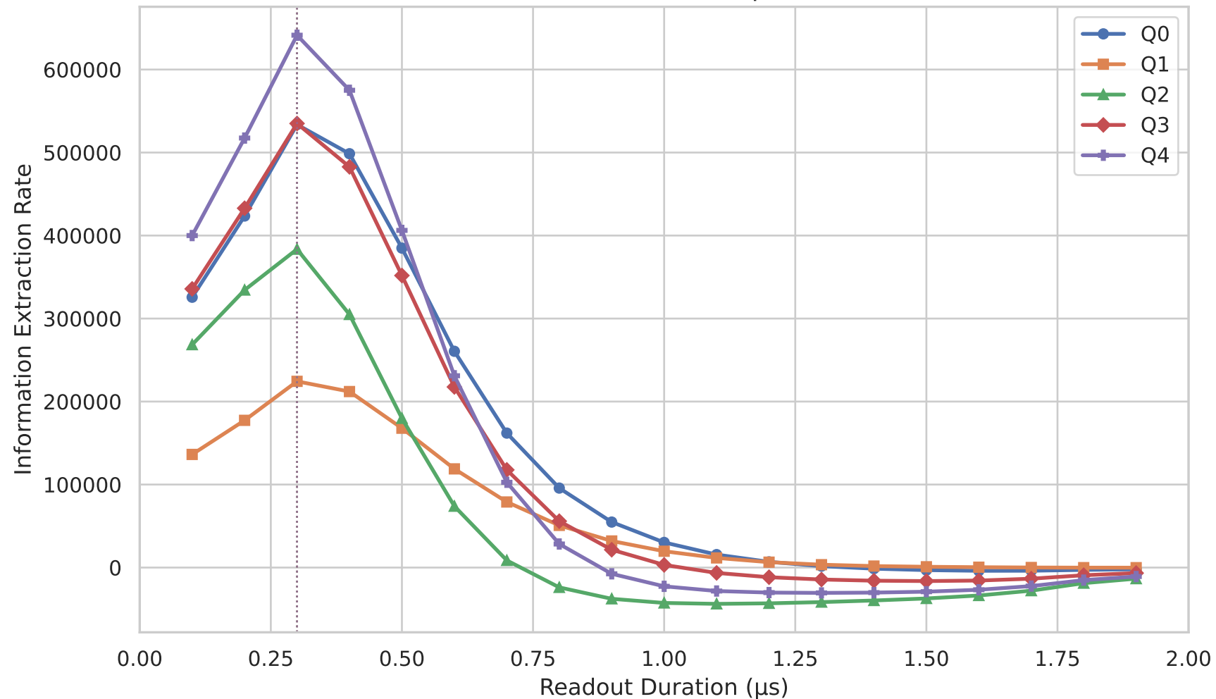
Information Gain Rate per Qubit
