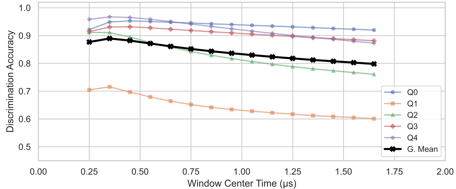
(b) Readout Window Effect on Accuracy - 500 ns Window
