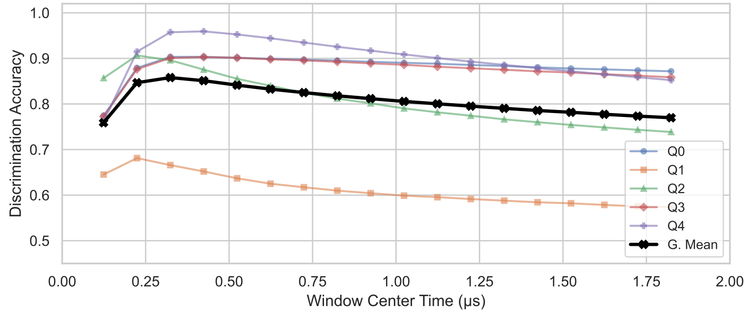
(a) Readout Window Effect on Accuracy - 250 ns Window
