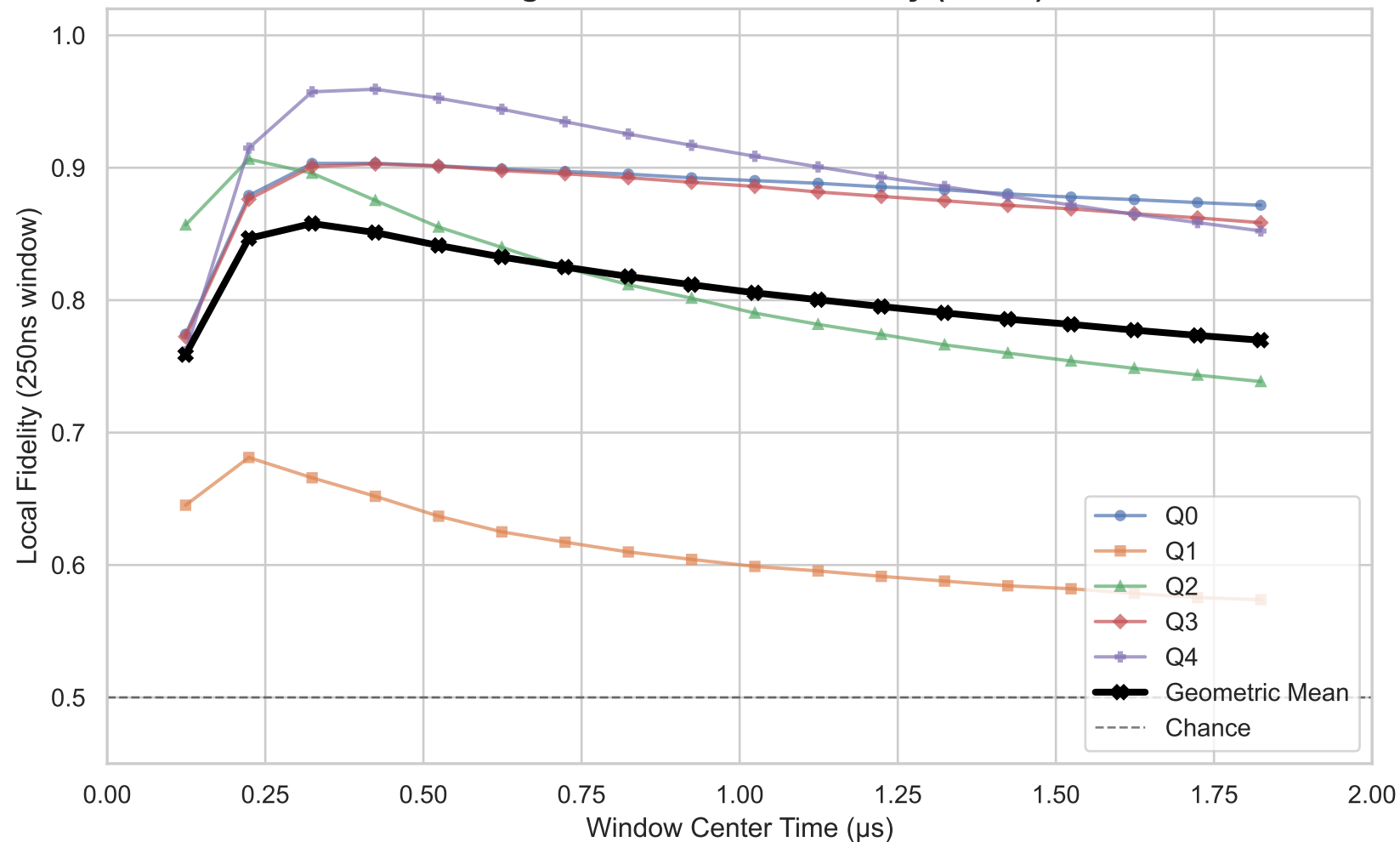
Sliding Window Readout Fidelity (250ns)
