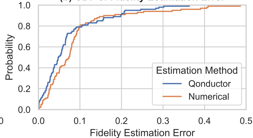
(b) CDF of Fidelity Estimation Error
