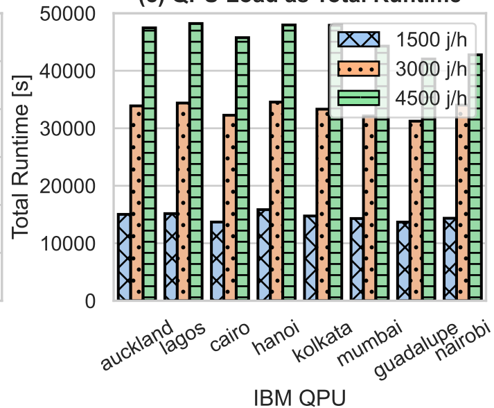
(c) QPU Load as Total Runtime
