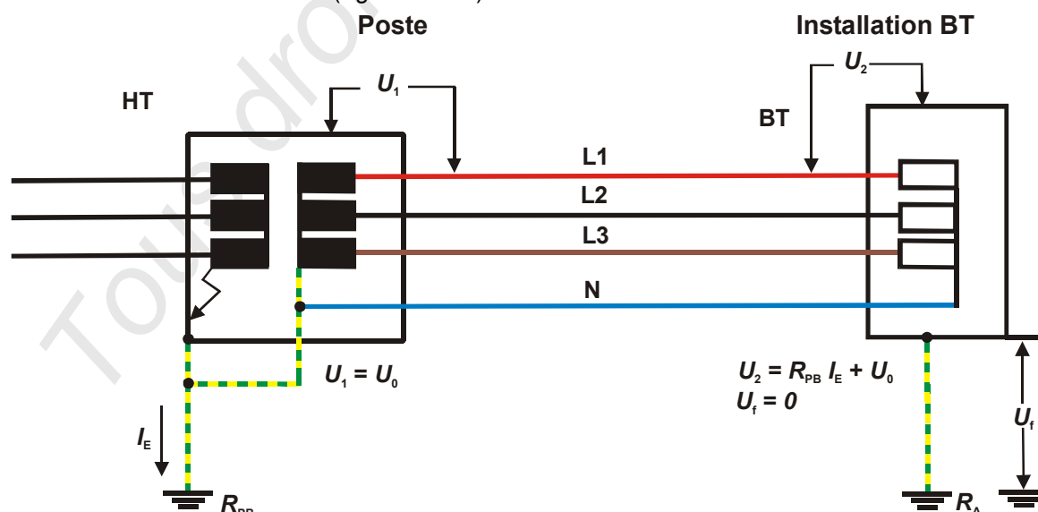
Figure 442C – Schéma TTN
