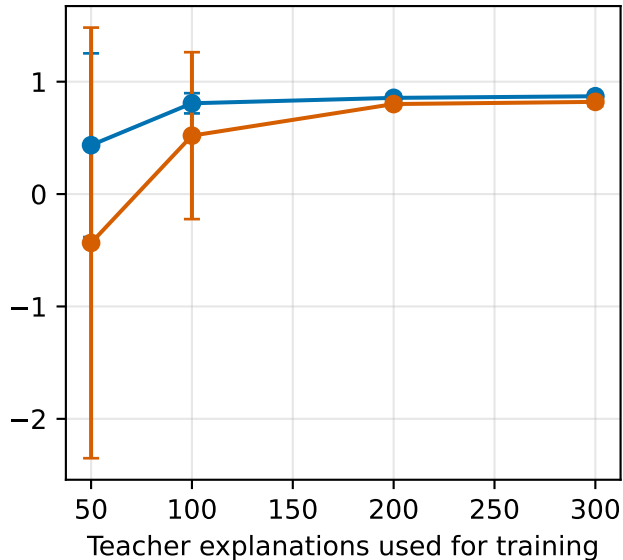
R^2 vs teacher
