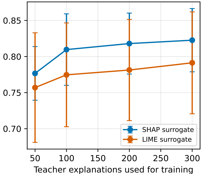
Top-3 overlap with teacher
