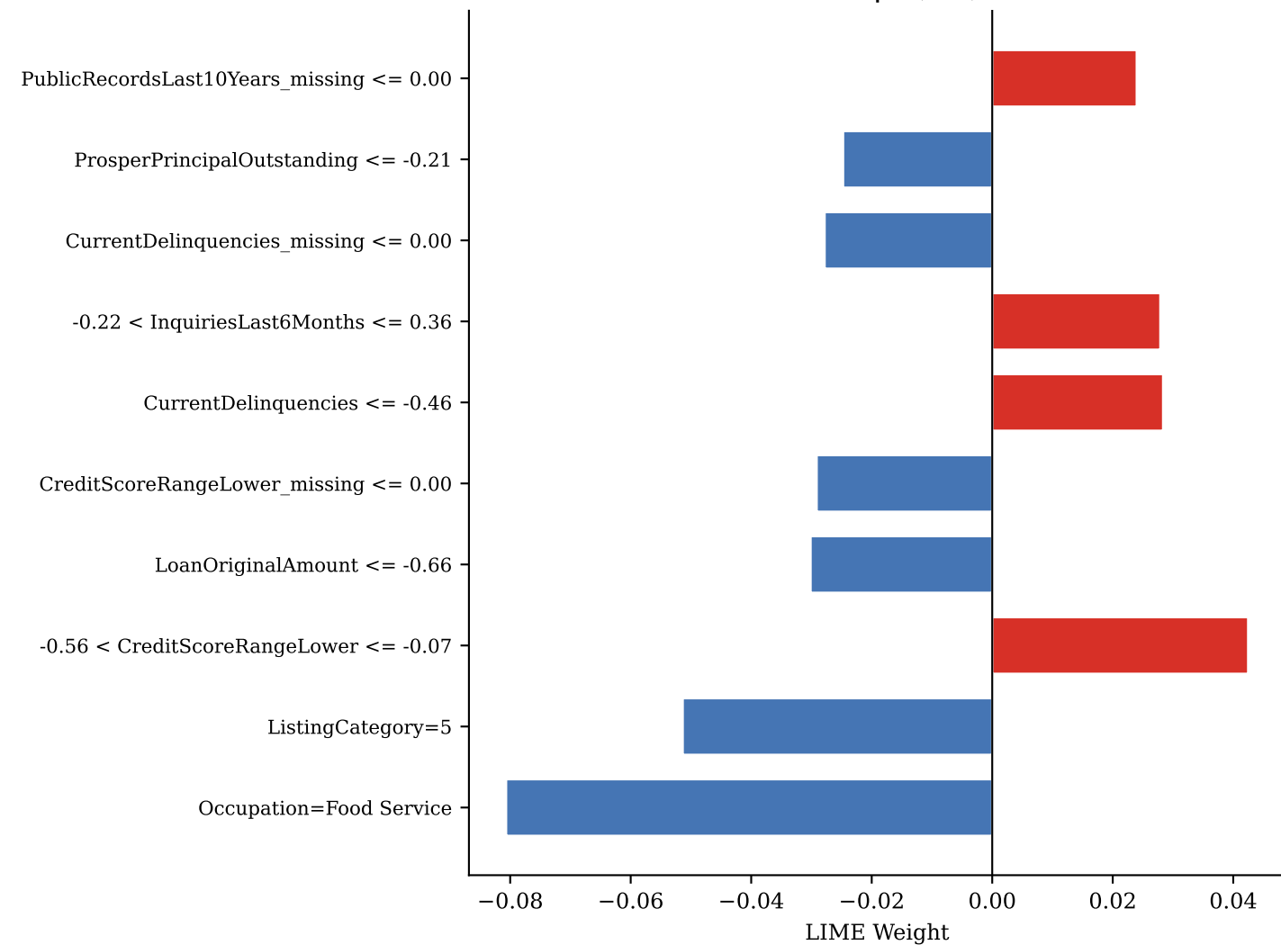
TN — idx 504 | P(def)=0.120
