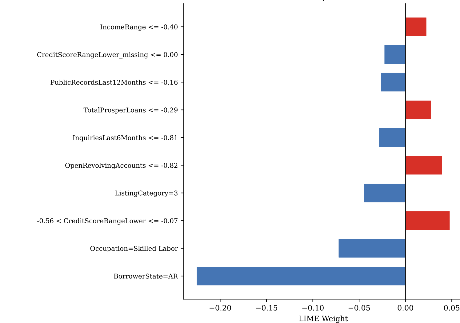
FN — idx 990 | P(def)=0.119
