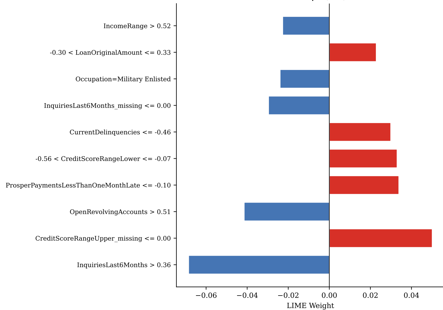
TN — idx 504 | P(def)=0.120
