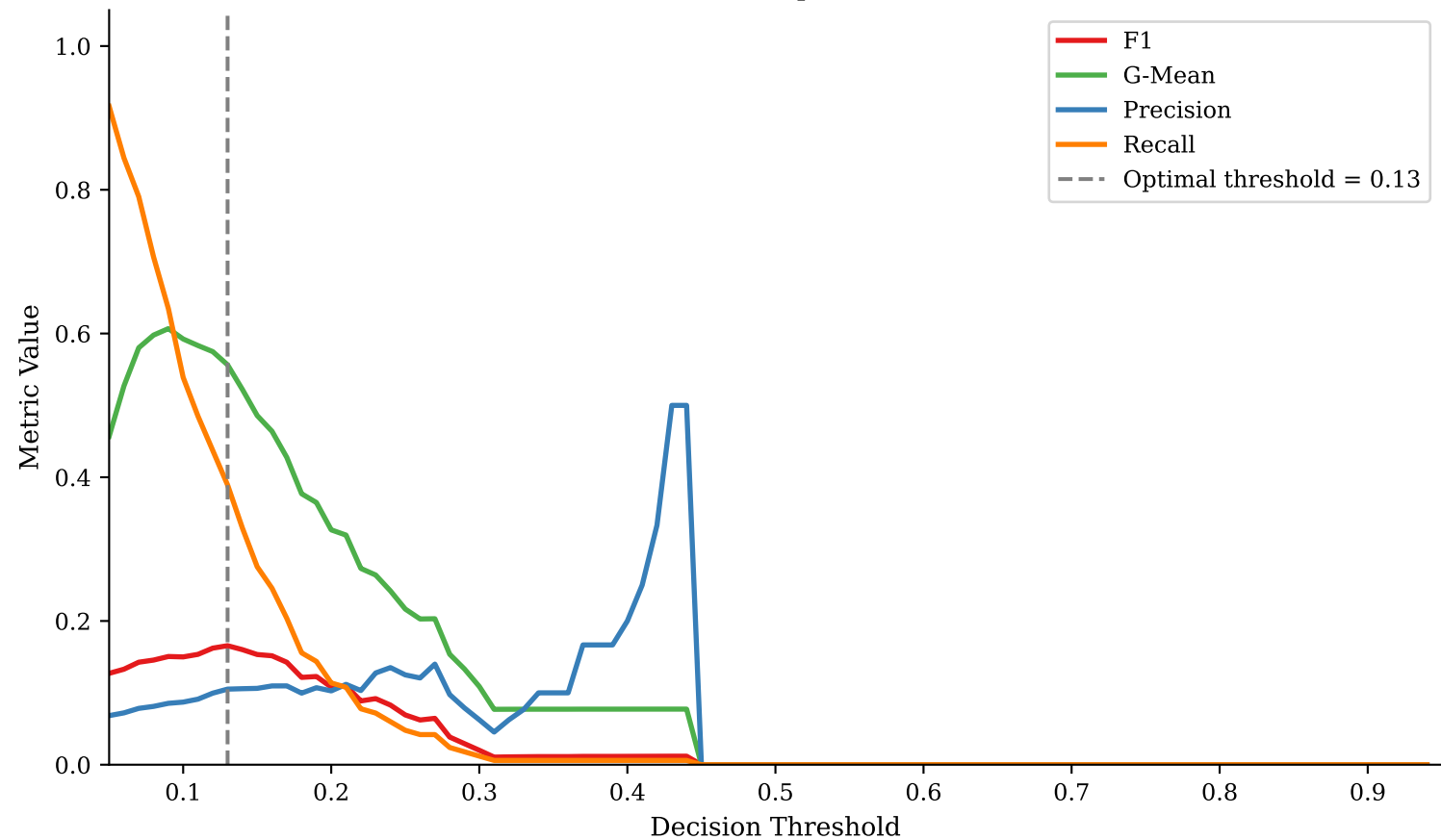
Threshold Sweep — XGBoost
