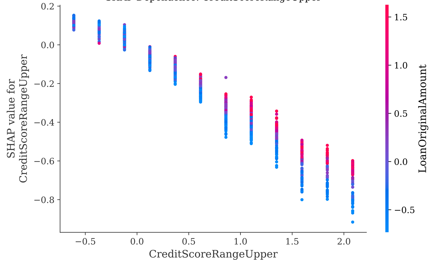
SHAP Dependence: CreditScoreRangeUpper
