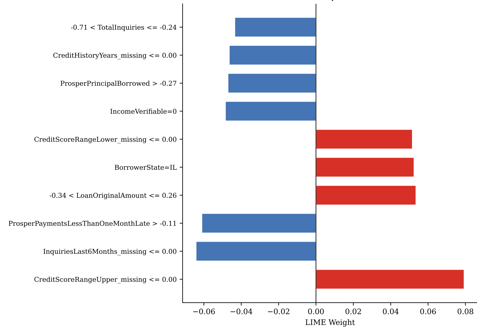
TN — idx 449 | P(def)=0.480
