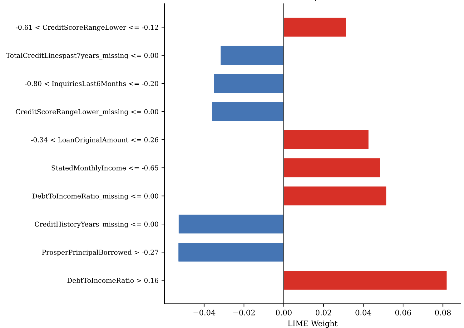
FN — idx 1549 | P(def)=0.480
