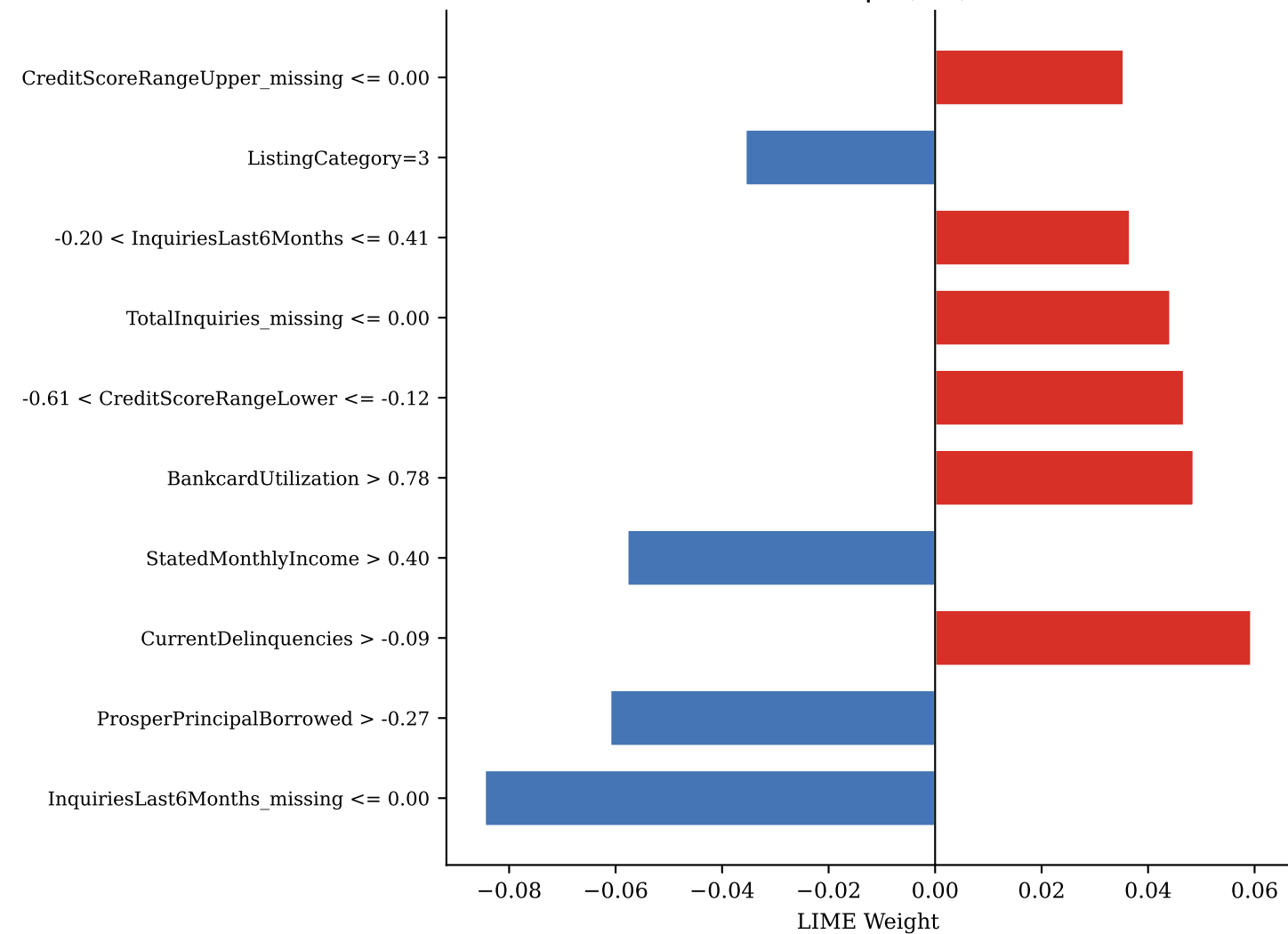
TN — idx 449 | P(def)=0.480
