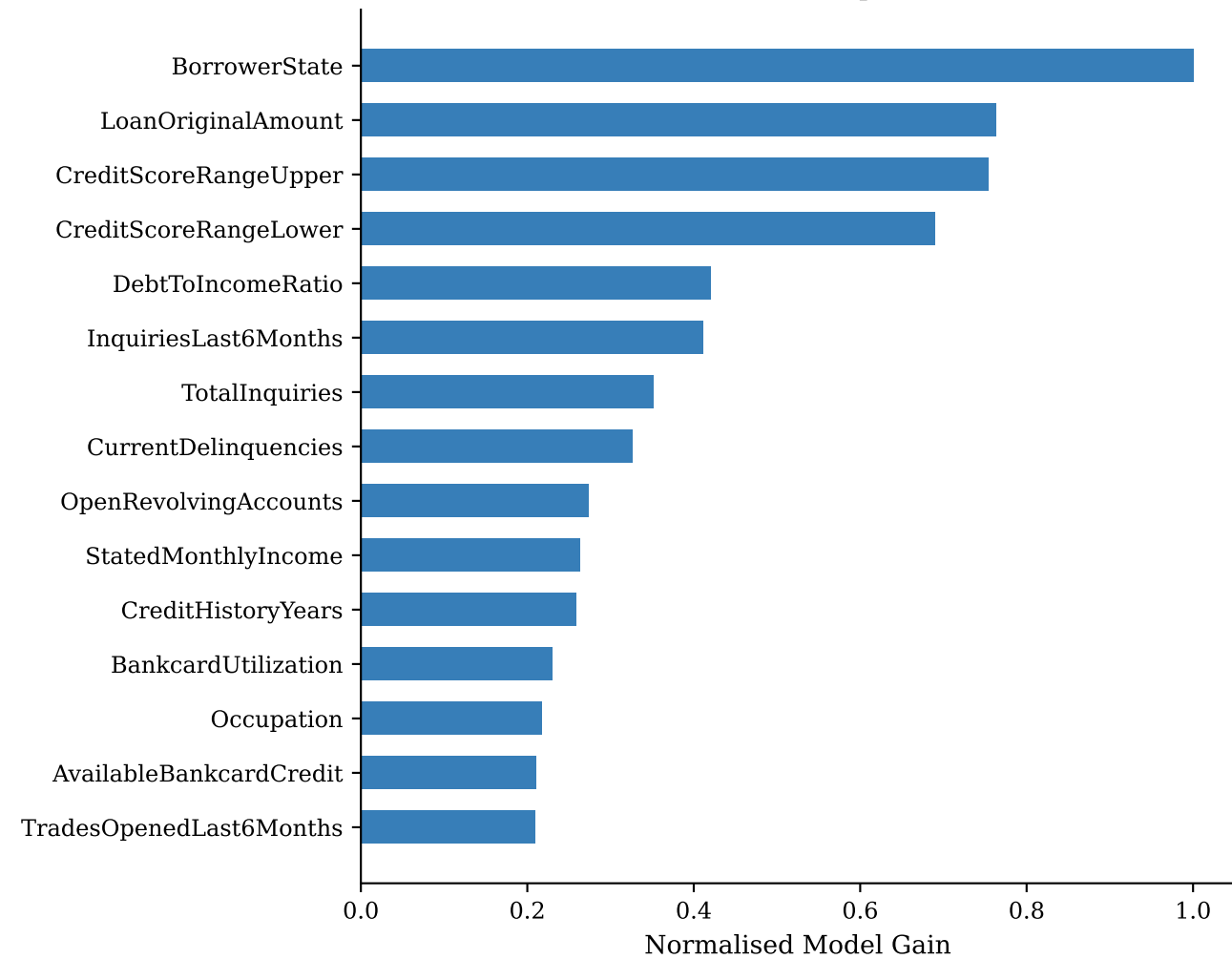
Model Built-in Importance
