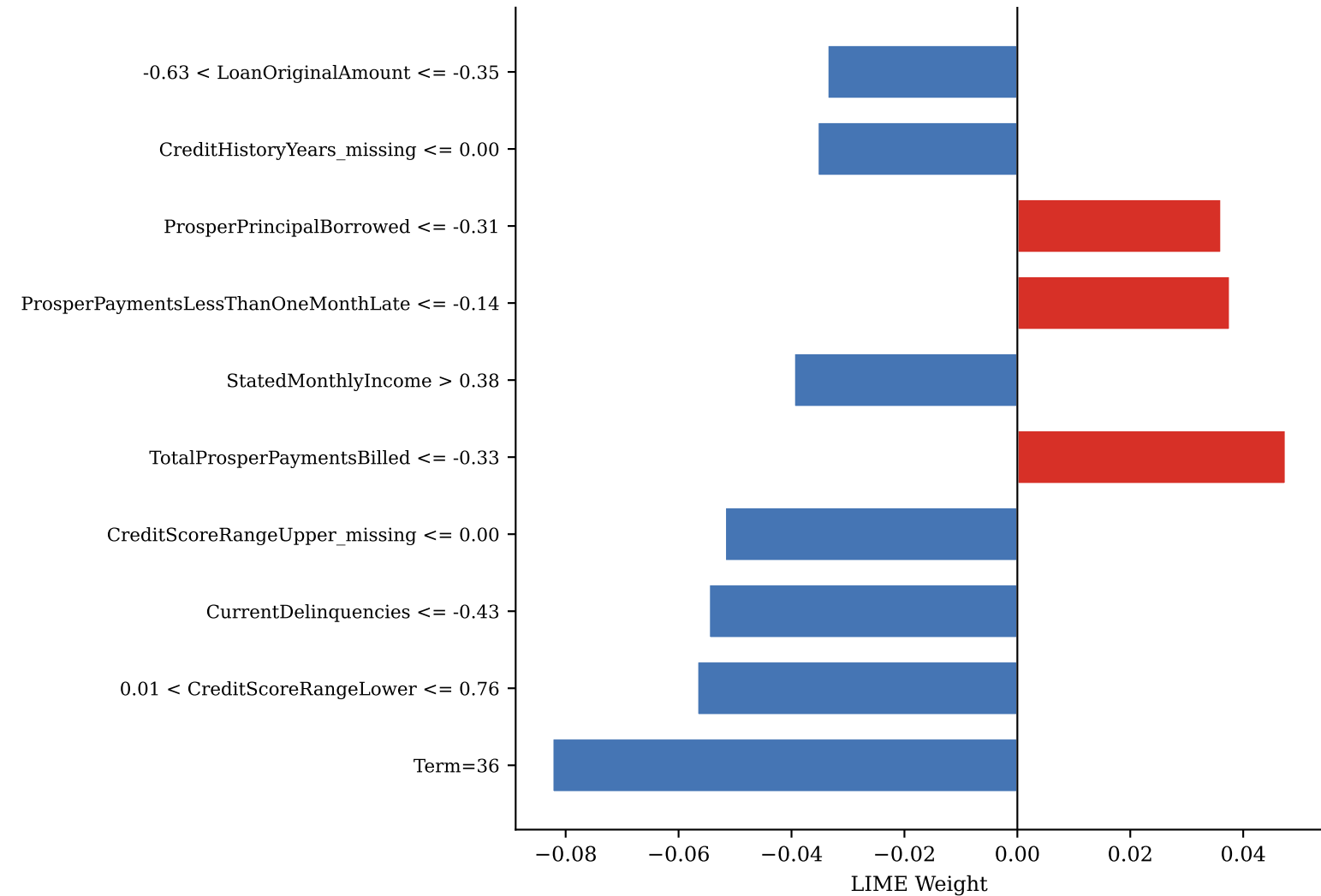
TN — idx 7808 | P(def)=0.410
