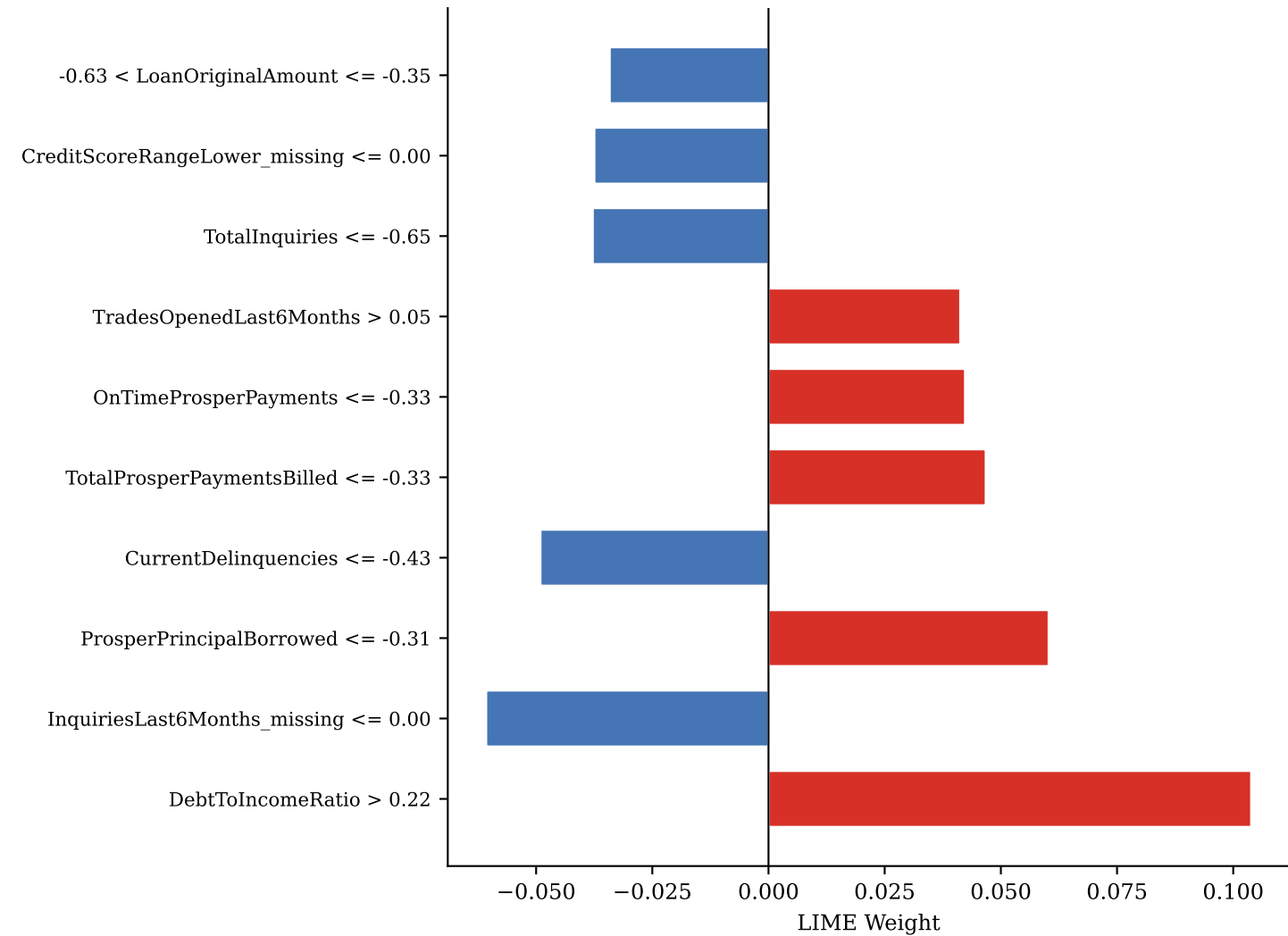
TN — idx 7808 | P(def)=0.410
