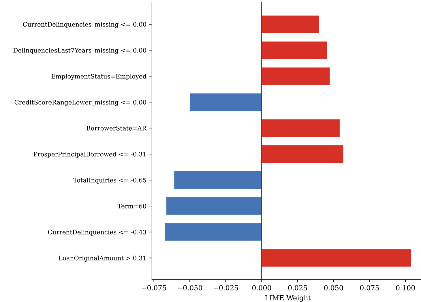
FN — idx 275 | P(def)=0.409
