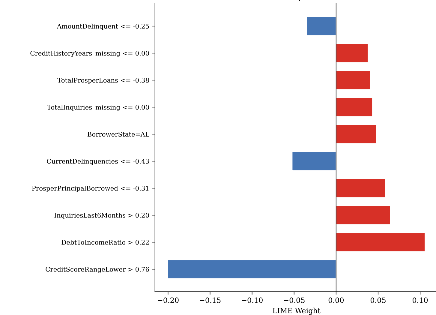
FN — idx 7171 | P(def)=0.410
