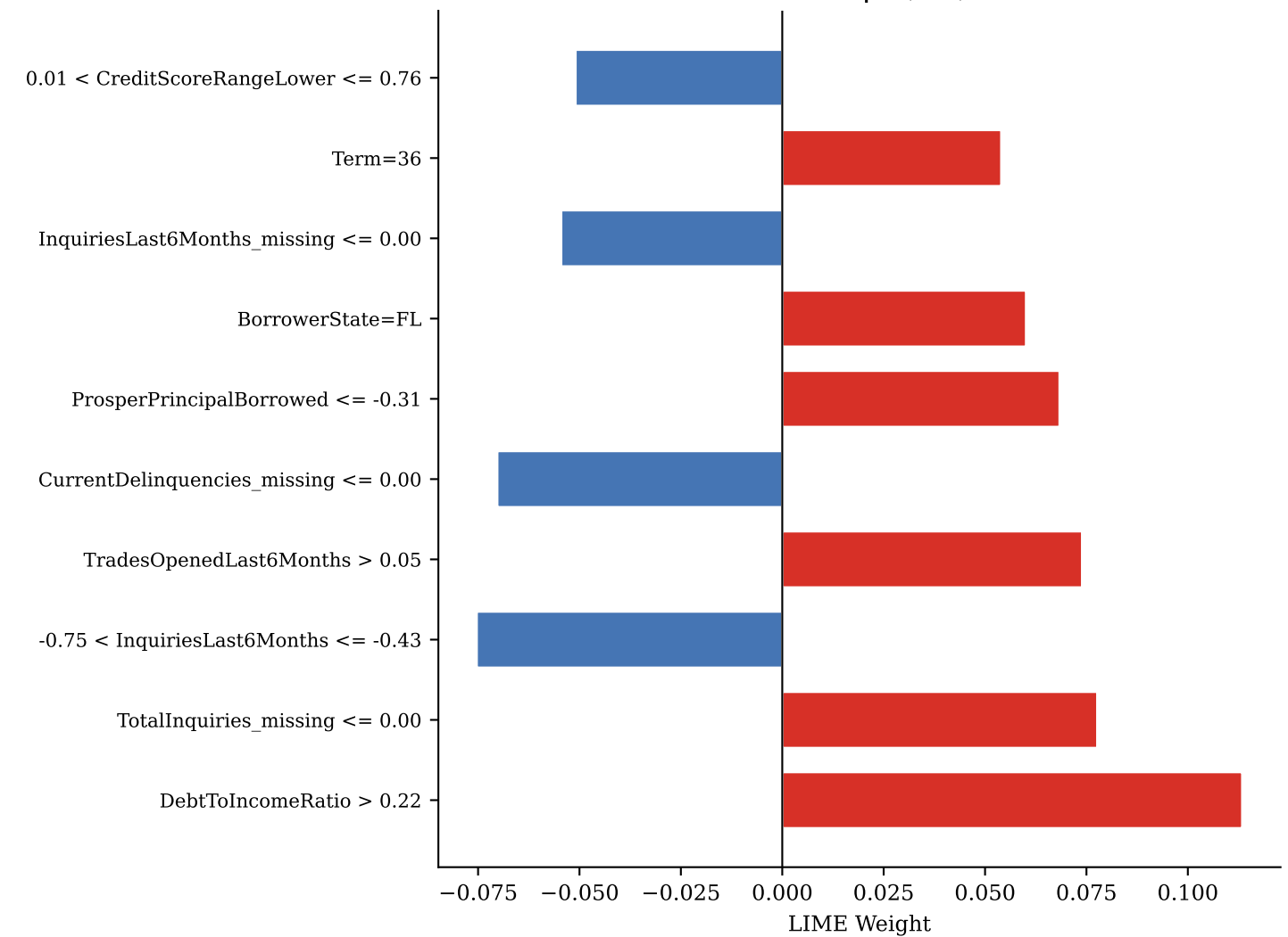
TN — idx 7581 | P(def)=0.410
