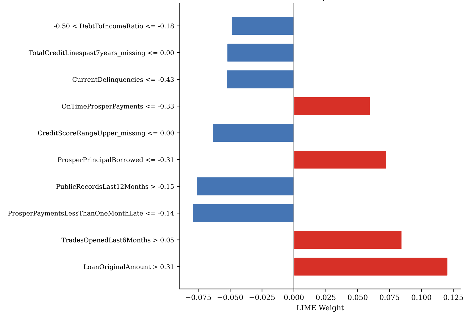
TN — idx 7581 | P(def)=0.410
