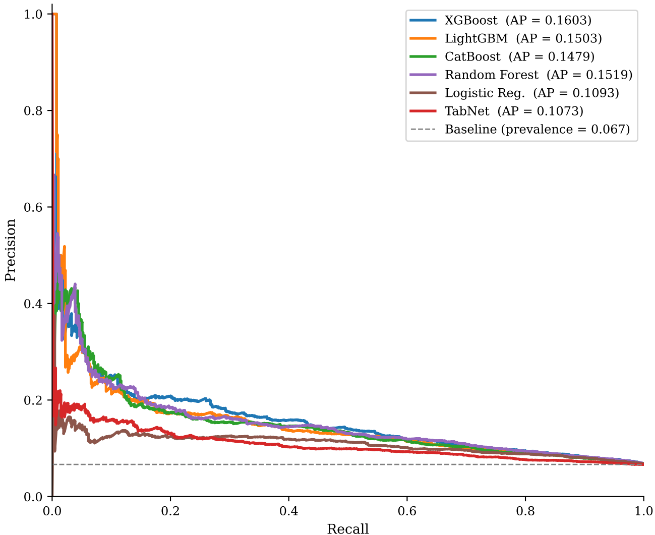
Precision-Recall Curves — All Models
