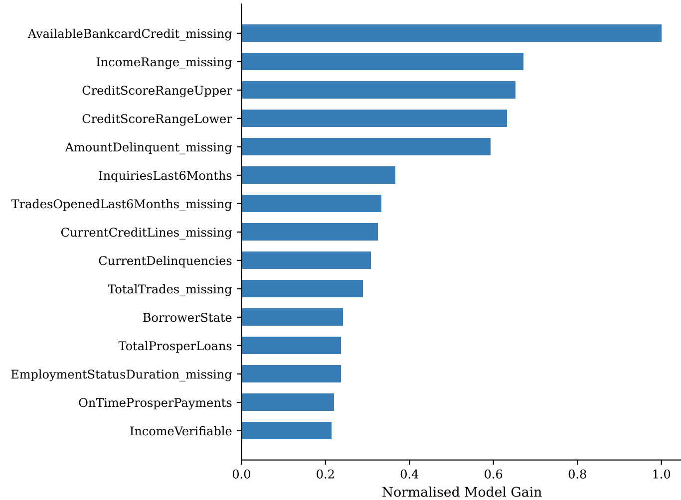
Model Built-in Importance
