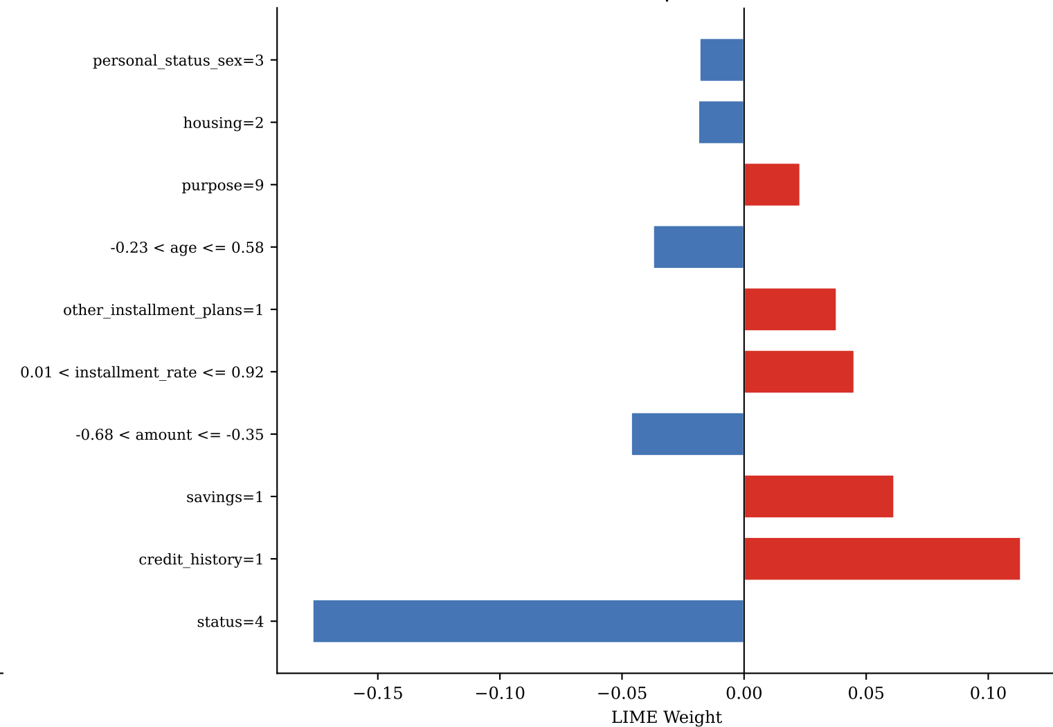
TN — idx 130 | P(def)=0.348
