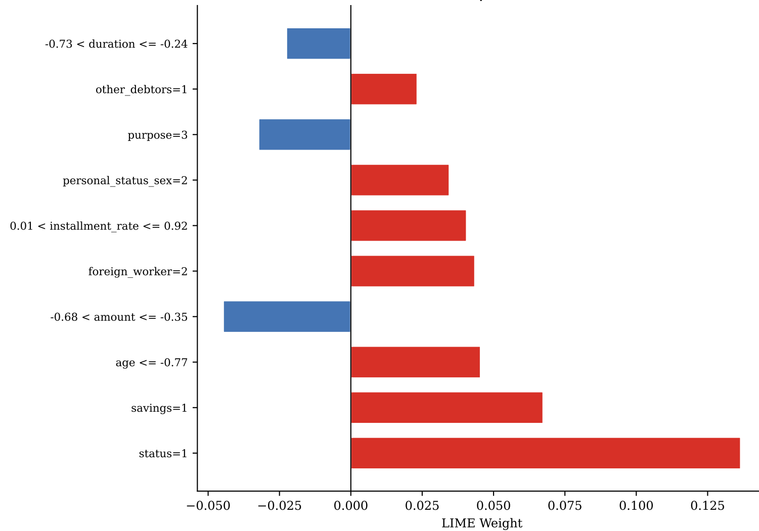
FN — idx 72 | P(def)=0.345
