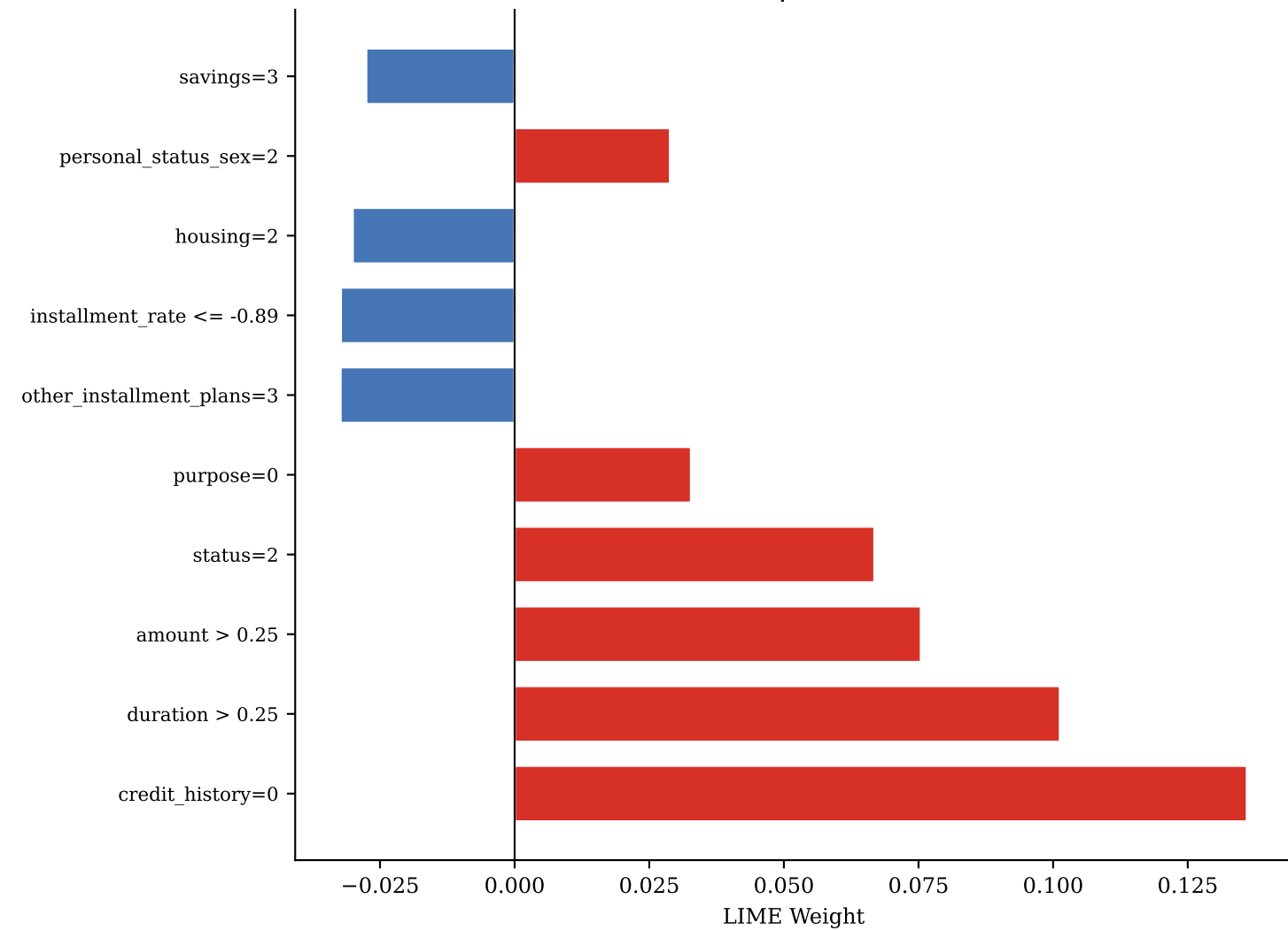
TN — idx 130 | P(def)=0.348
