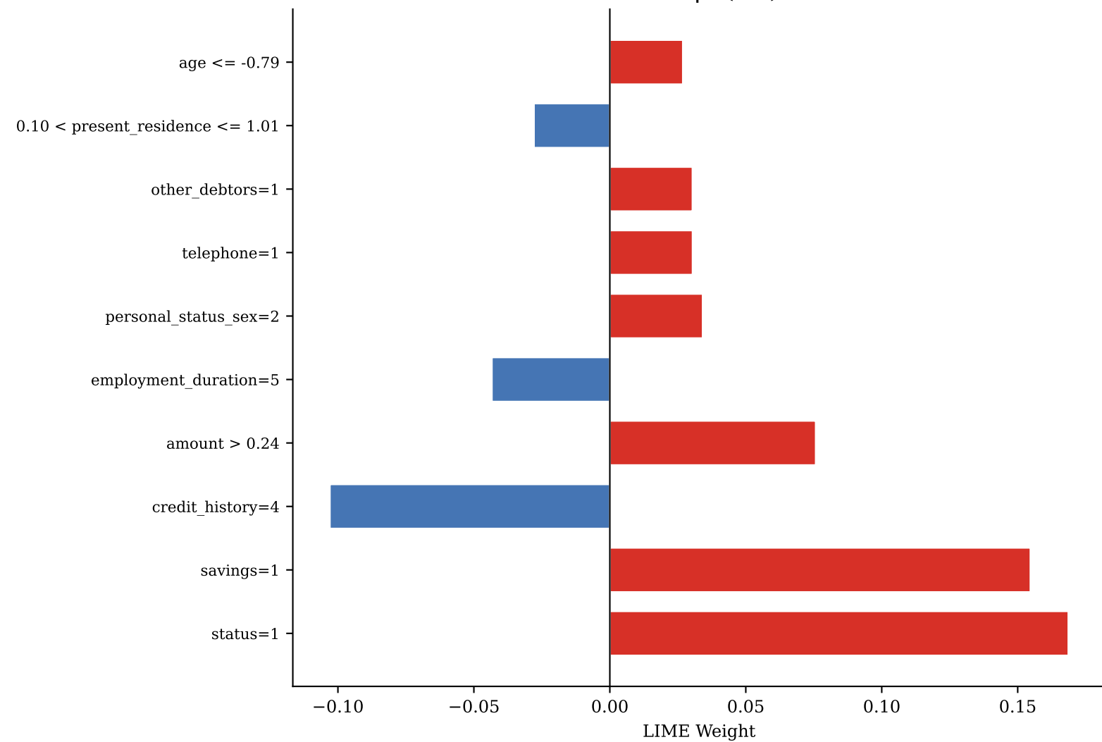
TN — idx 65 | P(def)=0.421
