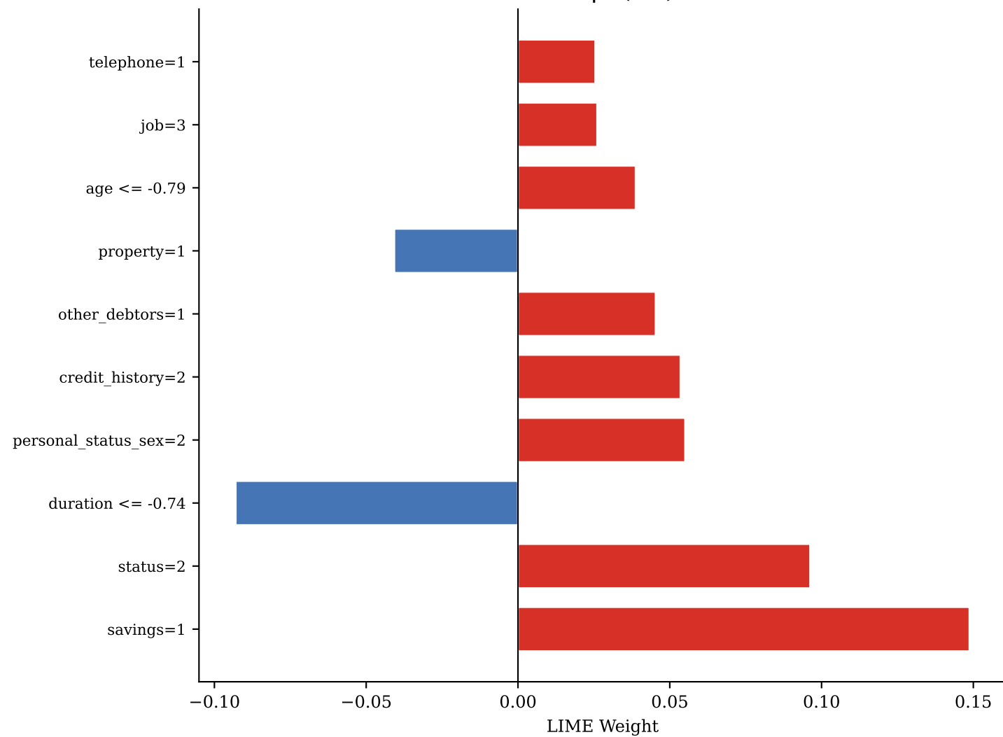
FN — idx 40 | P(def)=0.427
