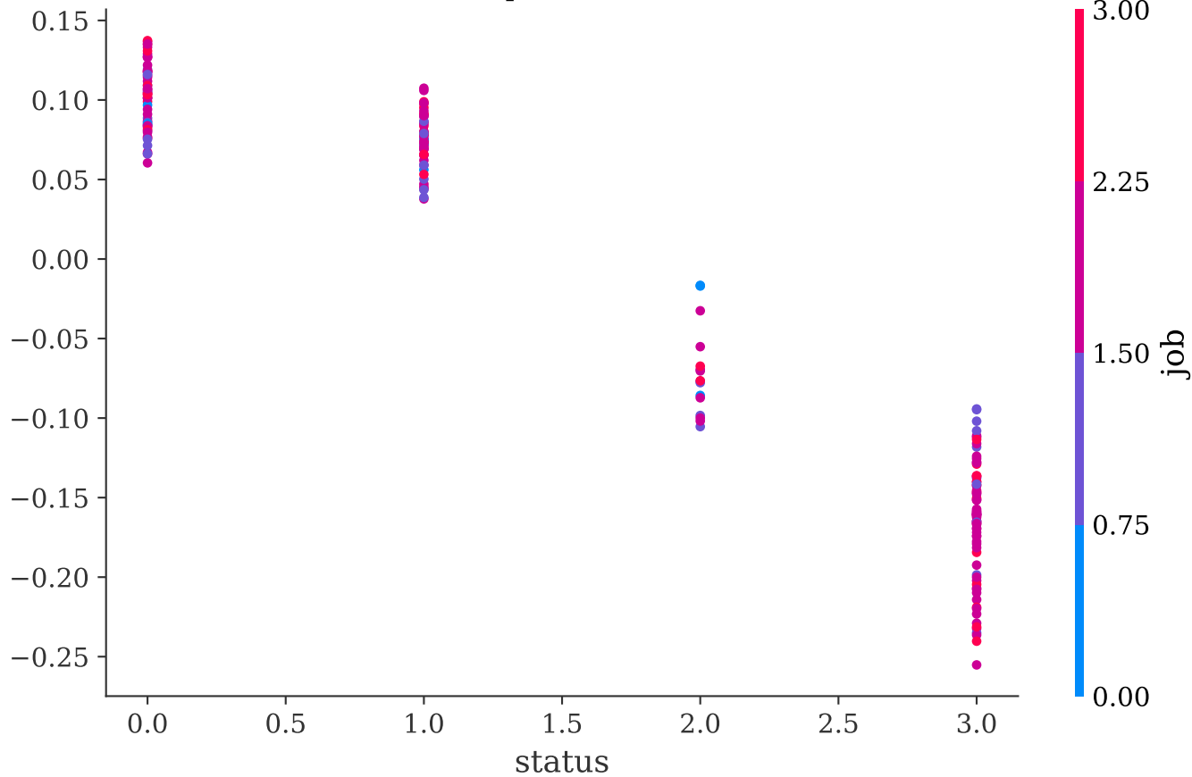
SHAP Dependence: status
