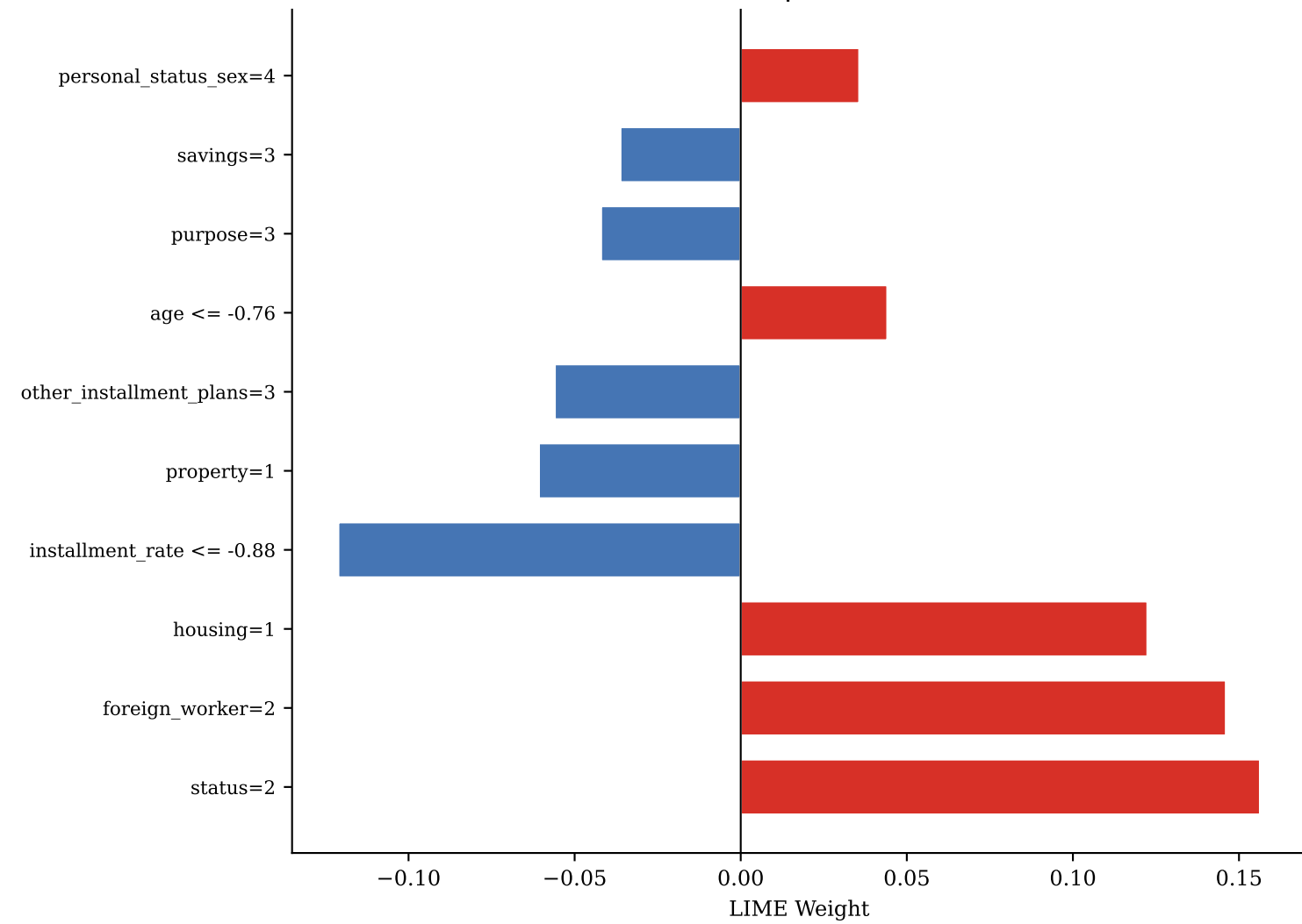
TN — idx 112 | P(def)=0.494
