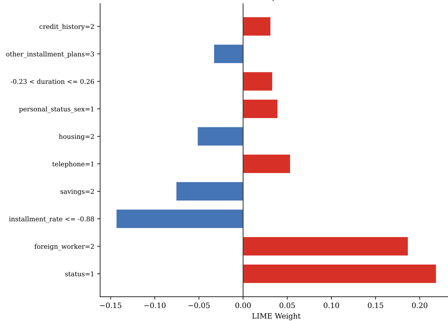
FN — idx 54 | P(def)=0.483
