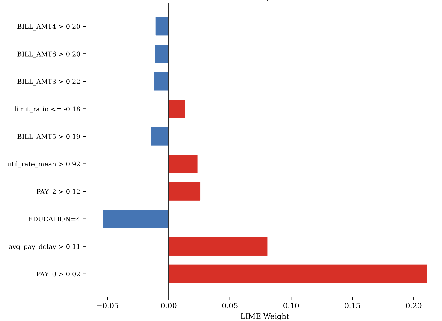
TN — idx 5847 | P(def)=0.289
