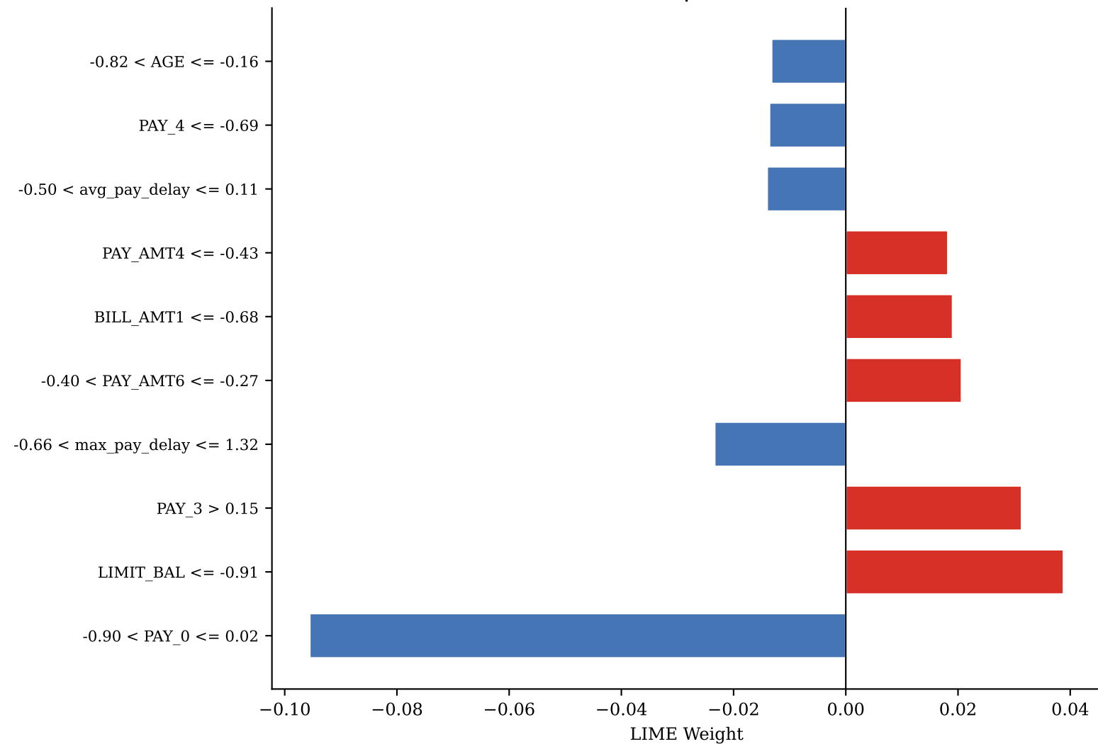
FN — idx 275 | P(def)=0.289
