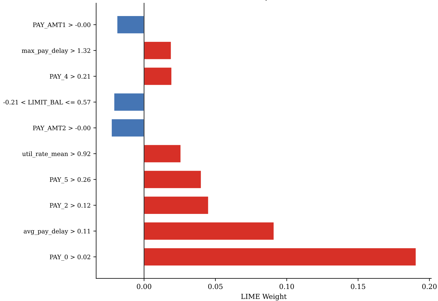
FN — idx 275 | P(def)=0.289
