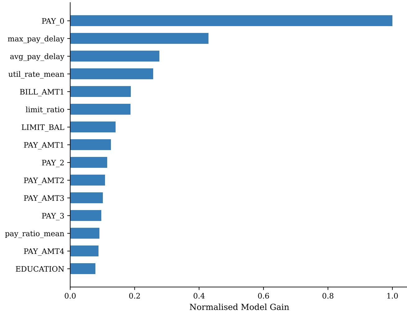
Model Built-in Importance
