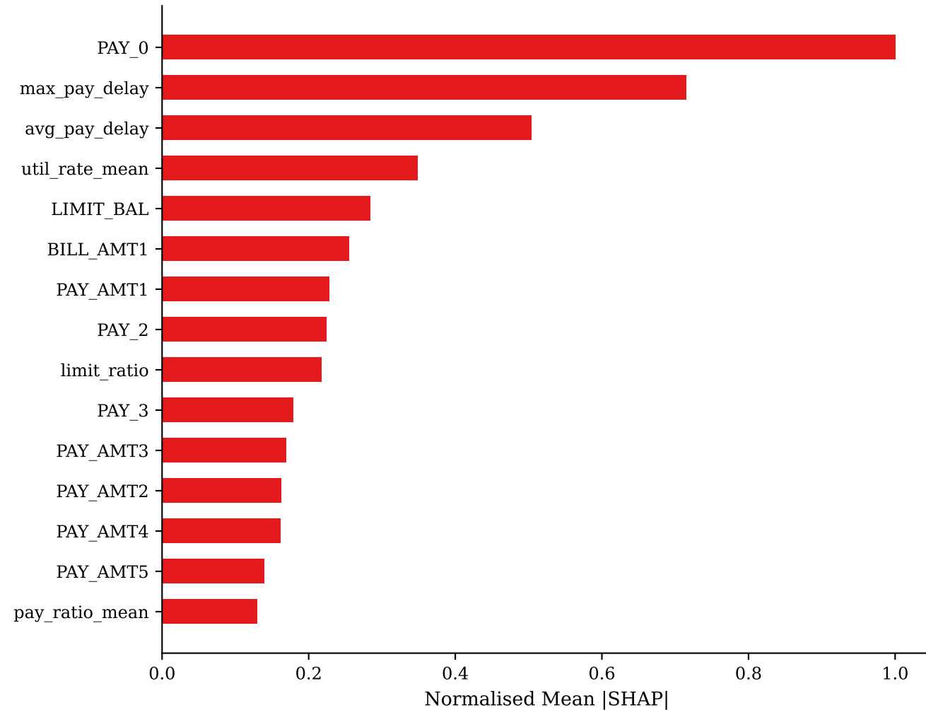
SHAP Feature Importance
