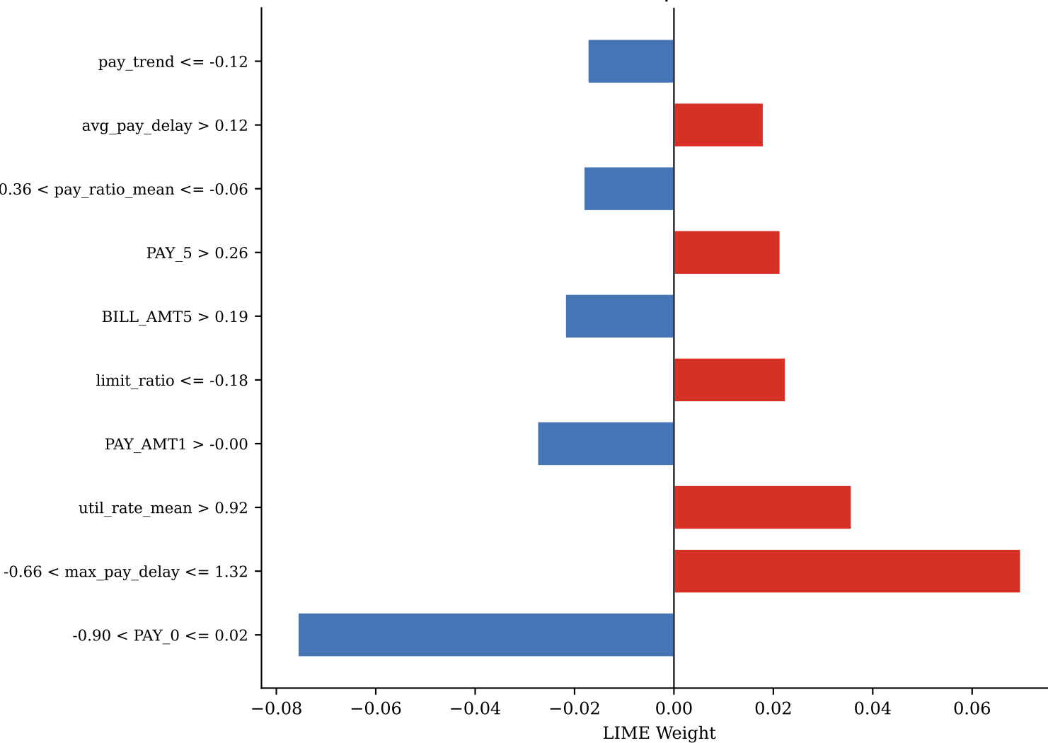
FN — idx 4485 | P(def)=0.500
