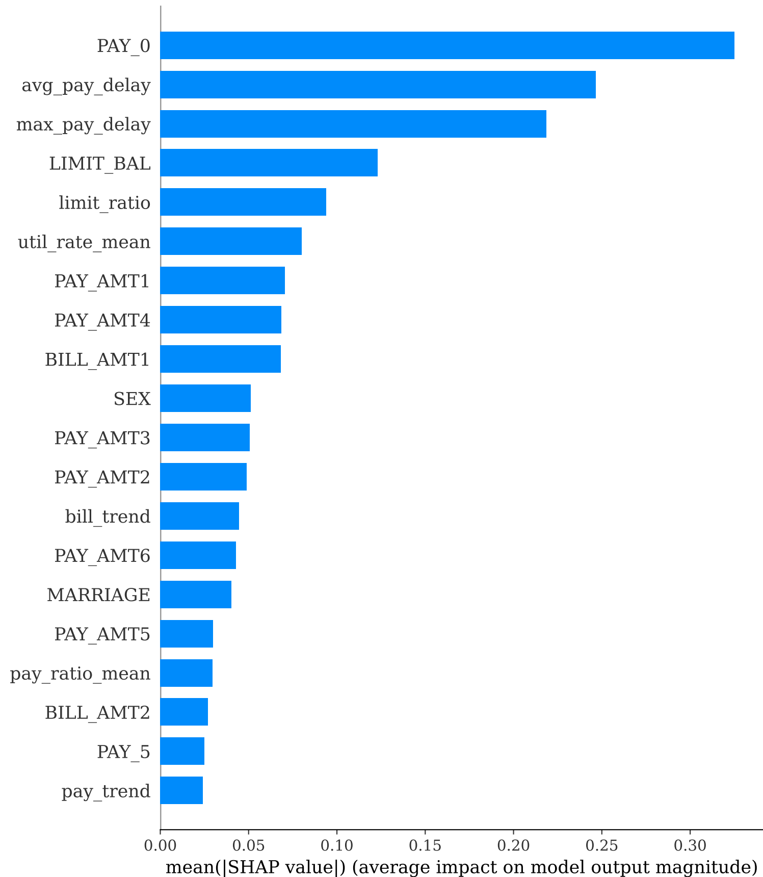
Mean |SHAP| — CatBoost
