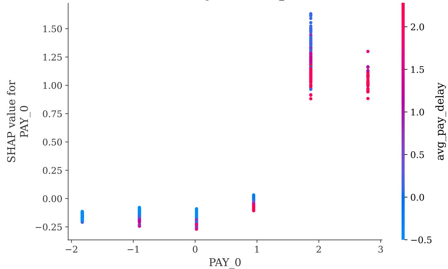
SHAP Dependence: PAY_0
