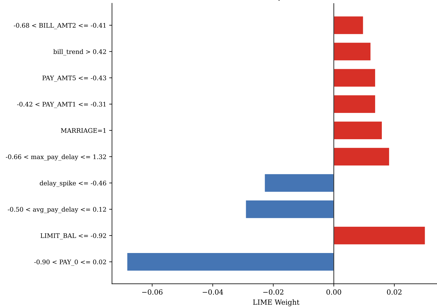
FN — idx 5344 | P(def)=0.280
