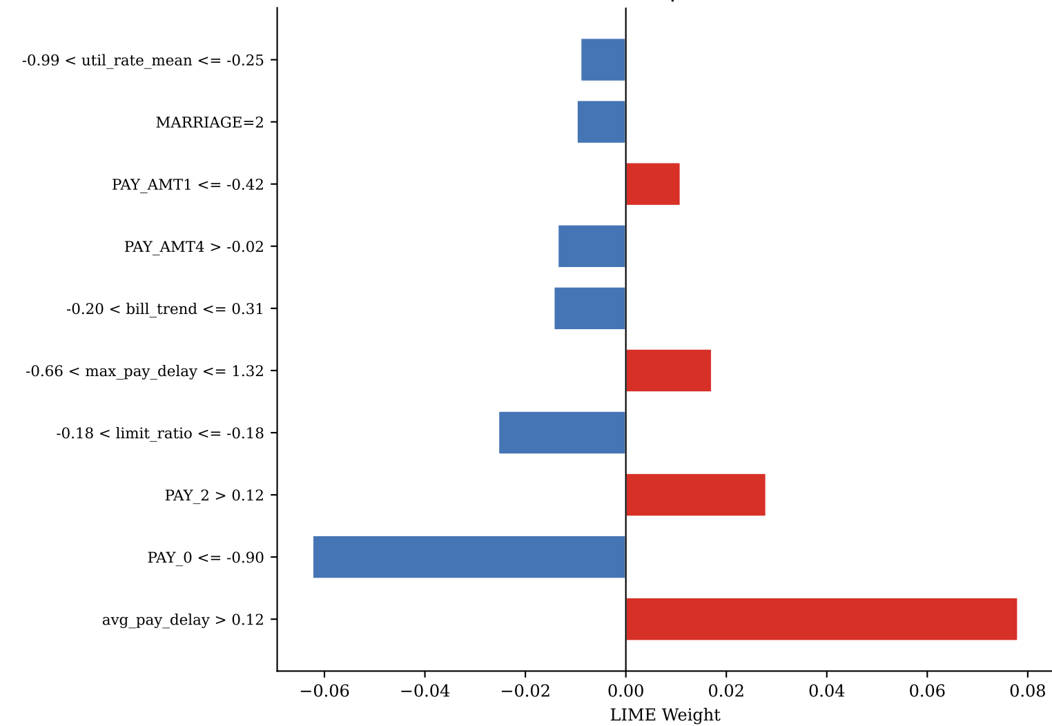
TN — idx 4391 | P(def)=0.280
