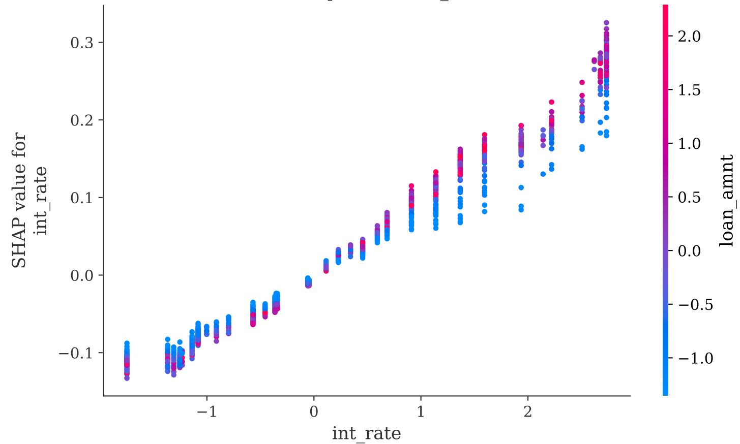
SHAP Dependence: int_rate
