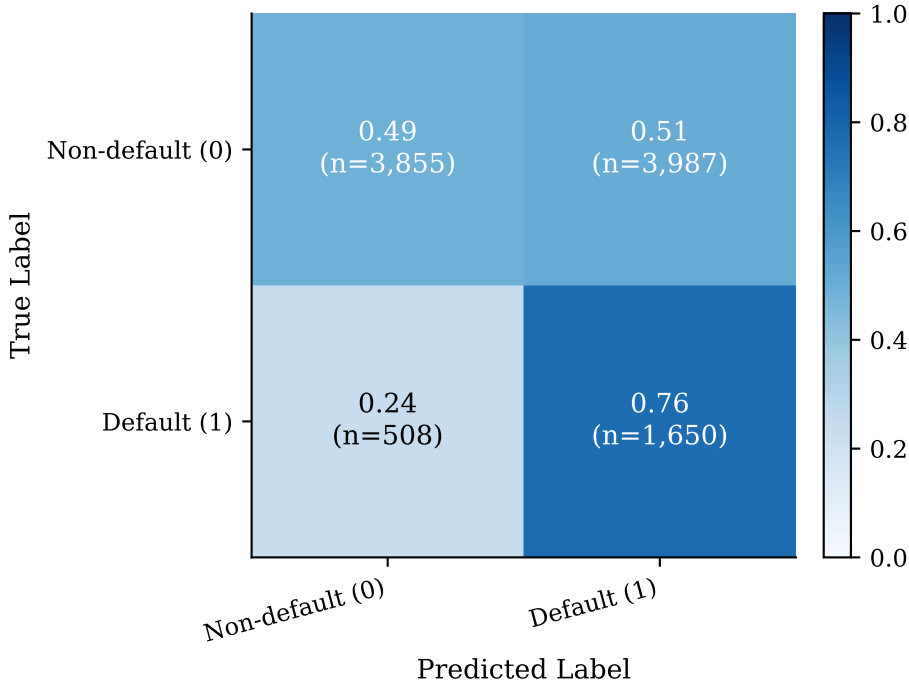
Confusion Matrix — CatBoost
