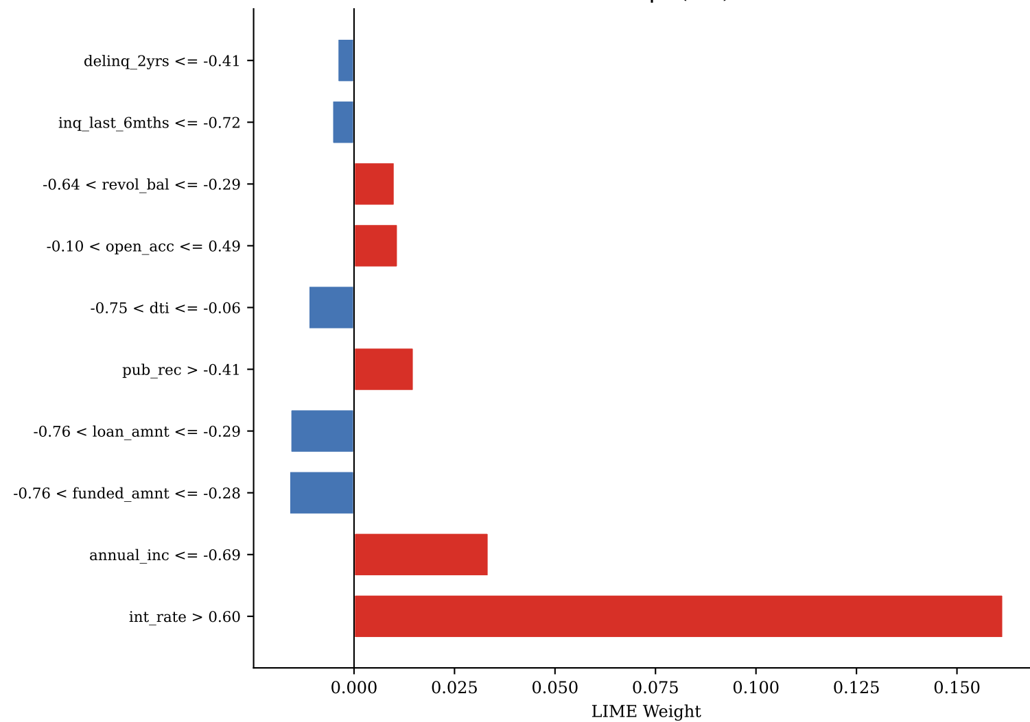
FN — idx 6367 | P(def)=0.150
