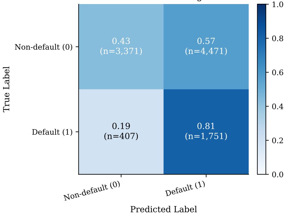
Confusion Matrix — LightGBM
