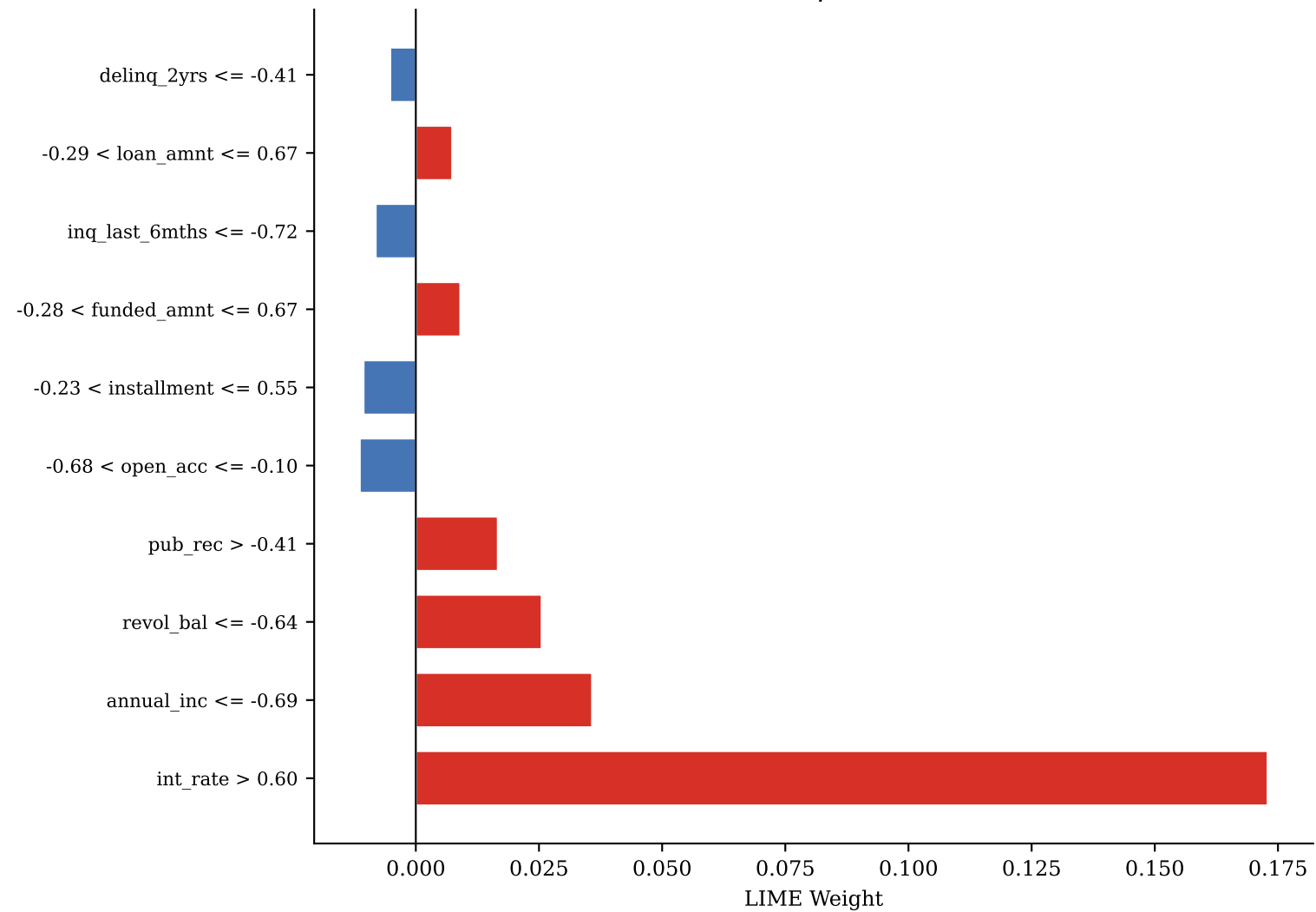
TN — idx 4931 | P(def)=0.160
