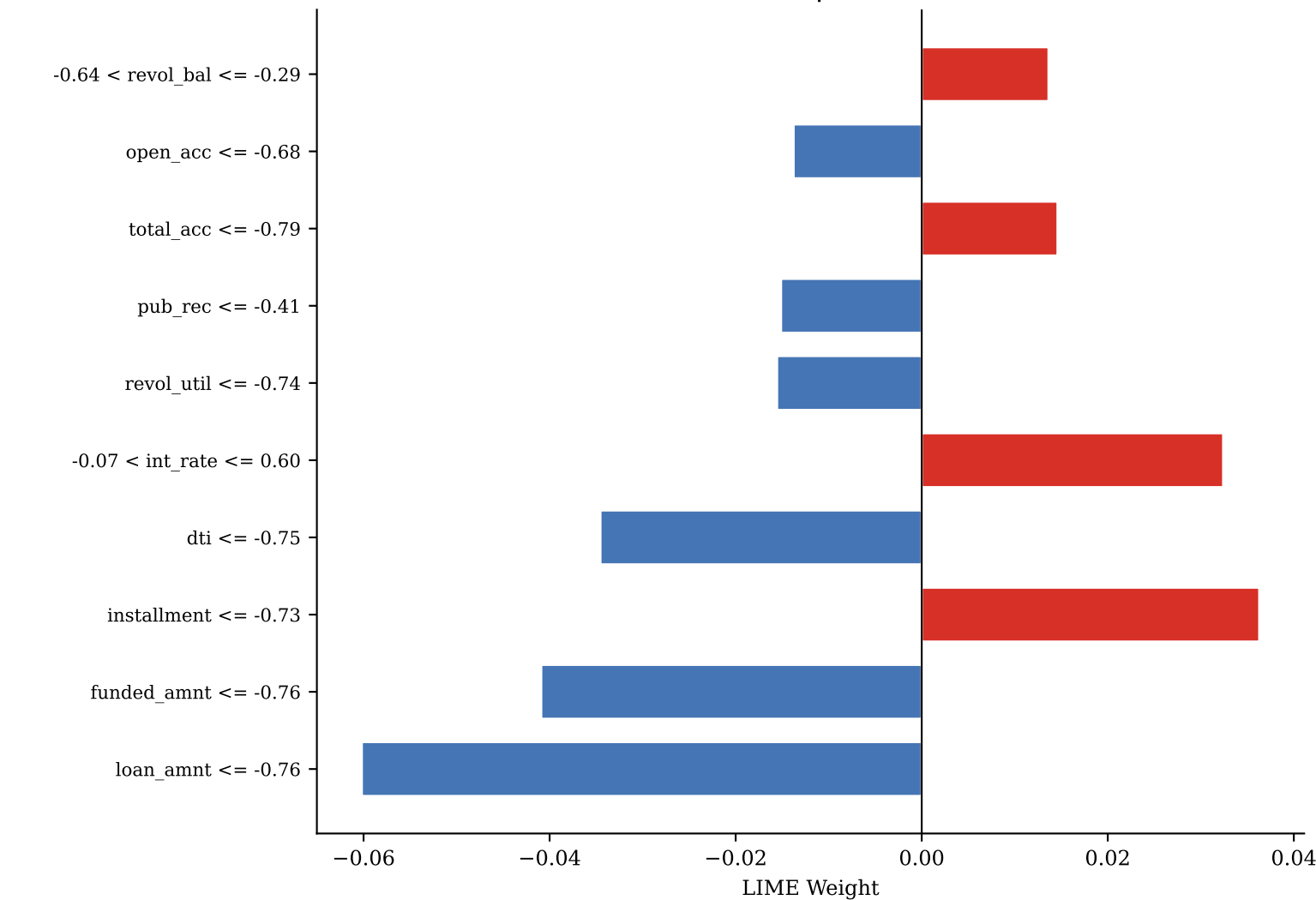
FN — idx 9321 | P(def)=0.160
