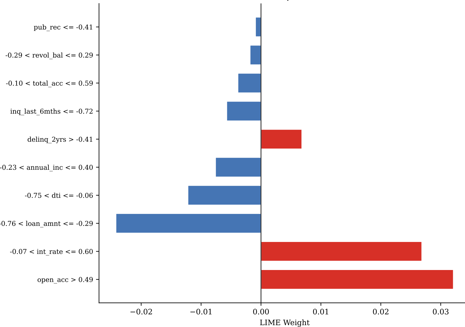
FN — idx 5126 | P(def)=0.160
