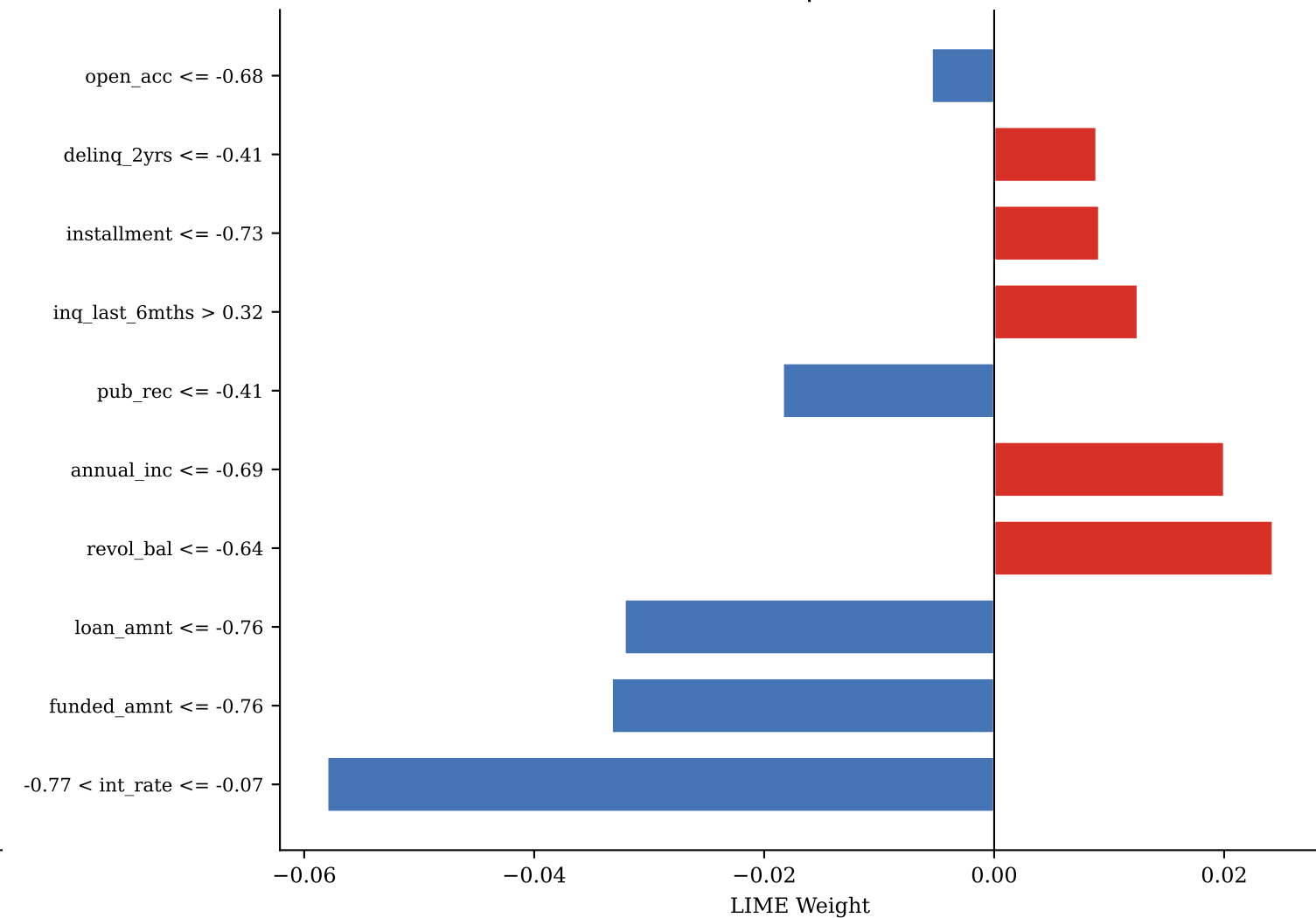
TN — idx 7214 | P(def)=0.160
