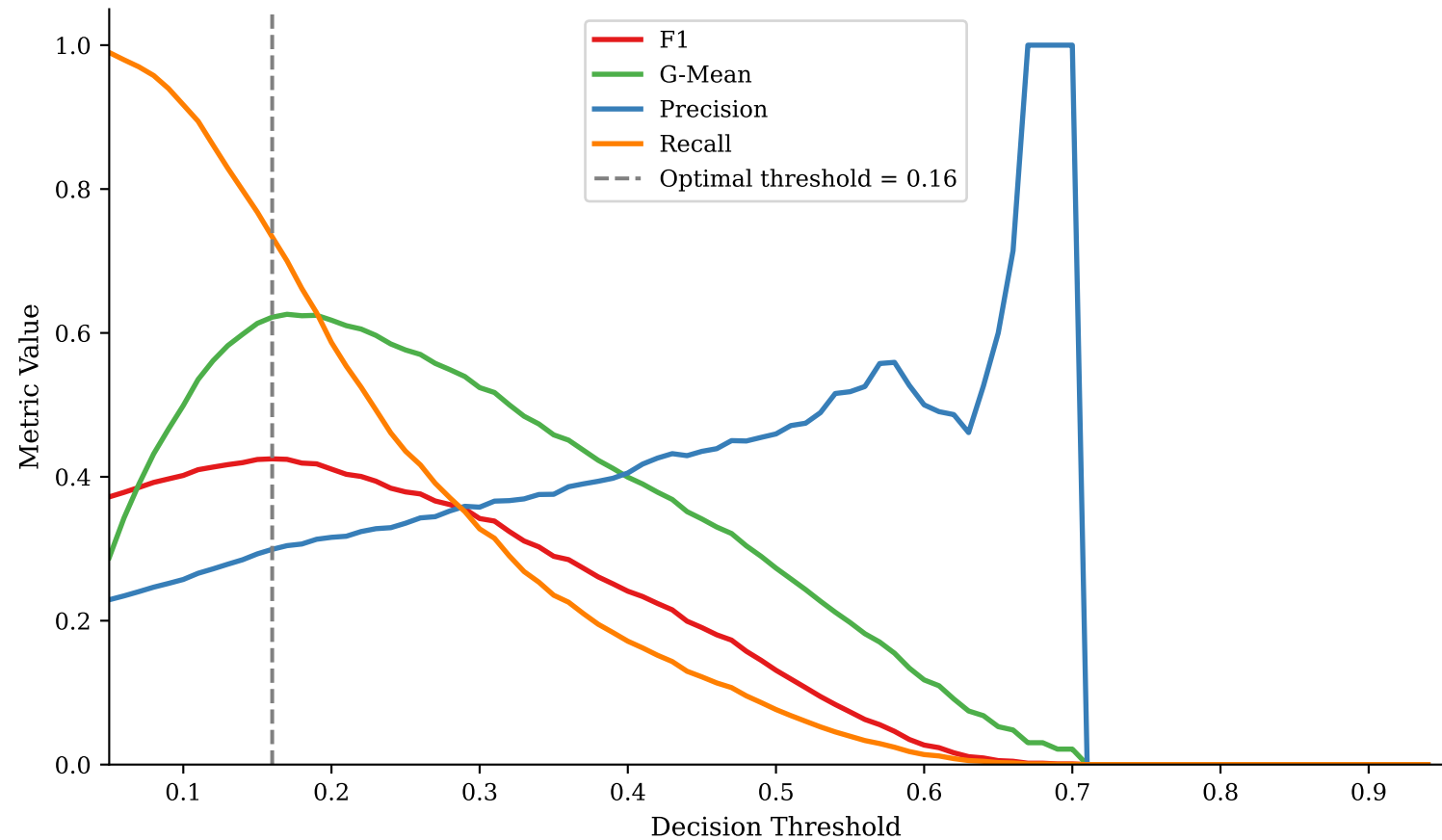
Threshold Sweep — CatBoost
